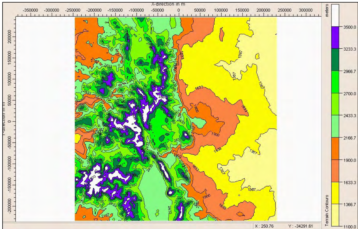
Figure 2. CALMET Terrain.
