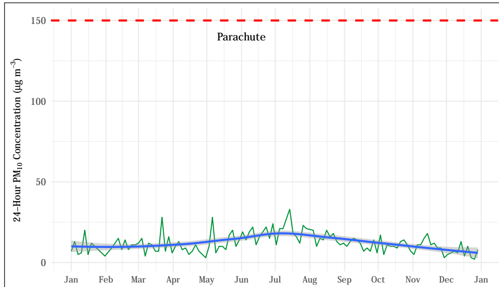
Figure 5.46: 24-hour average PM_{10} concentrations at the Parachute station. The mean trend obtained using a generalized additive model is shown as a blue line. The 24-hour standard ( 150 \mu\text{g m}^{-3} ) is shown as a dashed red line.
