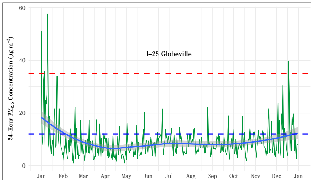
Figure 5.65: 24-hour average PM_{2.5} concentrations at the I-25 Globeville station. The mean trend obtained using a generalized additive model is shown as a blue line. The 24-hour standard ( 35 \mu\text{g m}^{-3} ) is shown as a dashed red line. The annual mean standard ( 12 \mu\text{g m}^{-3} ) is shown as a dashed blue line. The exceedances which took place in January and December have been flagged by the division as exceptional prolonged inversion events.
