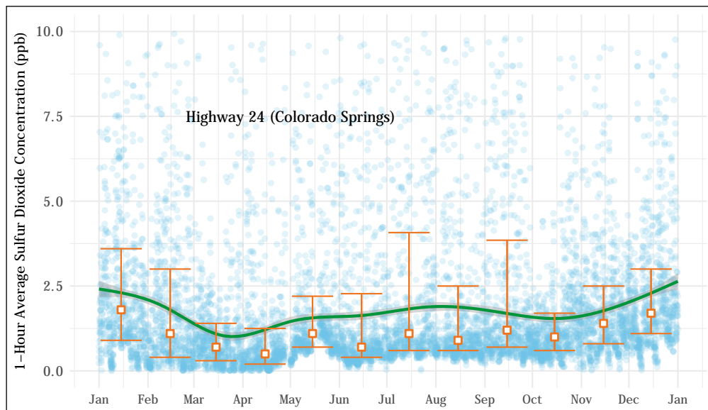
Figure 5.11: 1-hour average SO 2 concentrations at the Highway 24 (Colorado Springs) station (blue dots). The mean trend obtained using a generalized additive model is shown as a green line. The error bars represent the median and interquartile range of values observed during each month.
