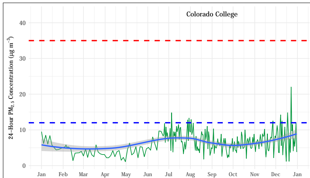
Figure 5.67: 24-hour average PM_{2.5} concentrations at the Colorado College station. The mean trend obtained using a generalized additive model is shown as a blue line. The 24-hour standard ( 35 \mu\text{g m}^{-3} ) is shown as a dashed red line. The annual mean standard ( 12 \mu\text{g m}^{-3} ) is shown as a dashed blue line.
