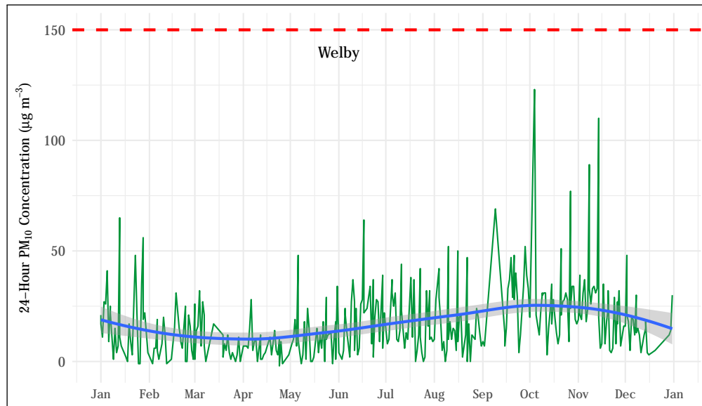
Figure 5.35: 24-hour average PM_{10} concentrations at the Welby station. The mean trend obtained using a generalized additive model is shown as a blue line. The 24-hour standard ( 150 \mu\text{g m}^{-3} ) is shown as a dashed red line.
