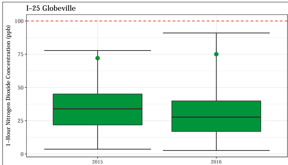
Figure 4.48: 1-hour average NO 2 concentrations at the I-25 Globeville station. The annual design value (98 th percentile of daily maximum 1-hour values) is shown for each year as a green point.
