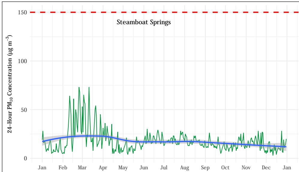
Figure 5.56: 24-hour average PM_{10} concentrations at the Steamboat Springs station. The mean trend obtained using a generalized additive model is shown as a blue line. The 24-hour standard ( 150 \mu\text{g m}^{-3} ) is shown as a dashed red line.
