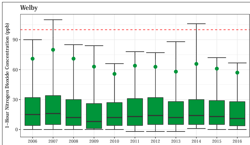
Figure 4.44: 1-hour average NO 2 concentrations at the Welby station. The annual design value (98 th percentile of daily maximum 1-hour values) is shown for each year as a green point.
