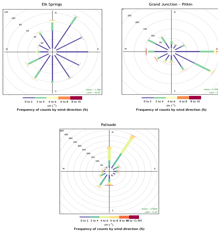
Figure 4.81: Wind roses for sites in the Western Slope Region during 2016.
