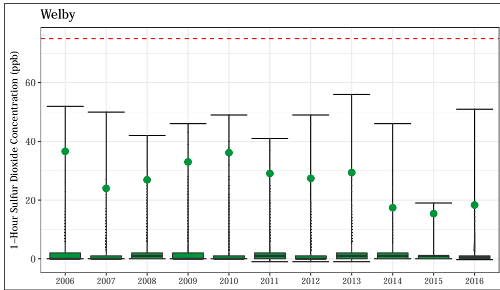
Figure 4.49: 1-hour average SO 2 concentrations at the Welby station. The annual design value (99 th percentile of daily maximum 1-hour values) is shown for each year as a green point.
