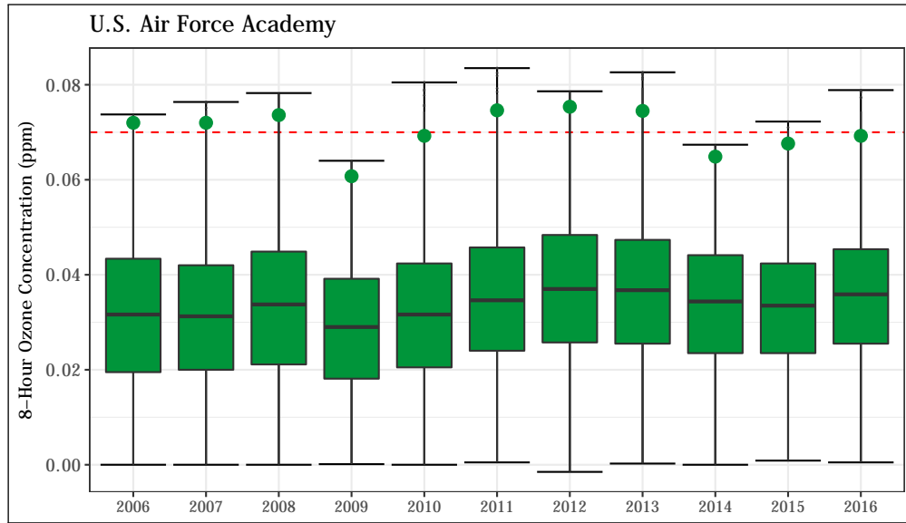
Figure 4.59: 8-hour average O 3 concentrations at the U.S. Air Force Academy station. The 8-hour standard (0.070 ppm) is shown as a dashed red line. The annual design value (4 th highest daily maximum 8-hour average value) is shown for each year as a green point.
