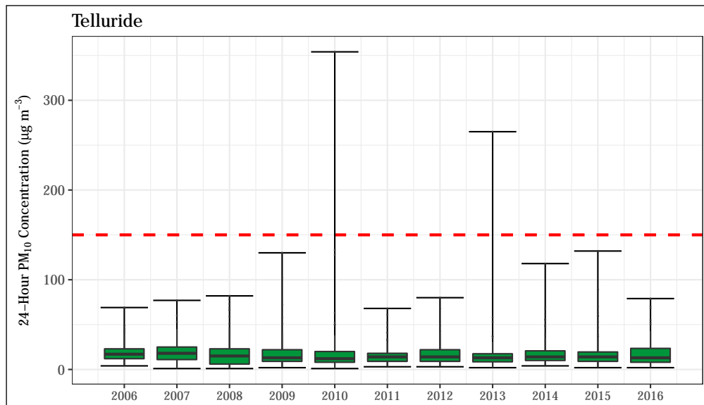
Figure 4.76: 24-hour average PM 10 concentrations at the Telluride station. The 24-hour standard (150 µg m -3 ) is shown as a dashed red line.
