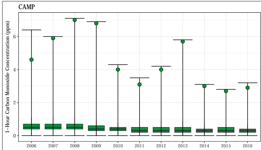
Figure 4.25: 1-hour average CO concentrations at the CAMP station. The annual design value (2 nd highest 1-hour value) is shown for each year as a green point.
