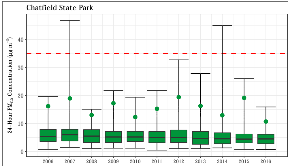
Figure 4.18: 24-hr PM 2.5 concentrations at the Chatfield station. The 24-hour standard (35 µg m -3 ) is shown as a dashed red line. The annual design value (98 th percentile of values measured throughout the year) is shown for each year as a green point.
