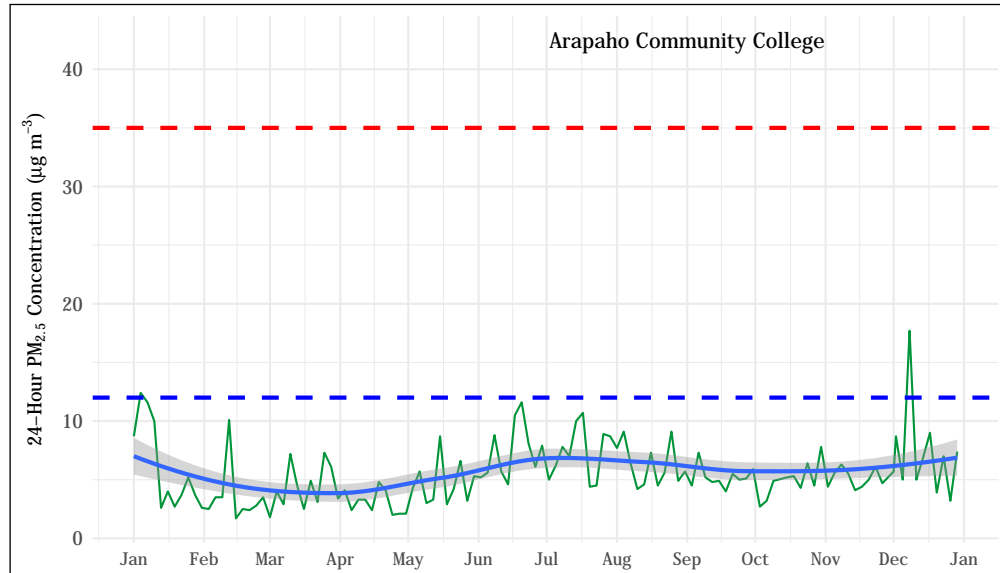
Figure 5.59: 24-hour average PM_{2.5} concentrations at the Arapaho Community College station. The mean trend obtained using a generalized additive model is shown as a blue line. The 24-hour standard ( 35 \mu\text{g m}^{-3} ) is shown as a dashed red line. The annual mean standard ( 12 \mu\text{g m}^{-3} ) is shown as a dashed blue line.
