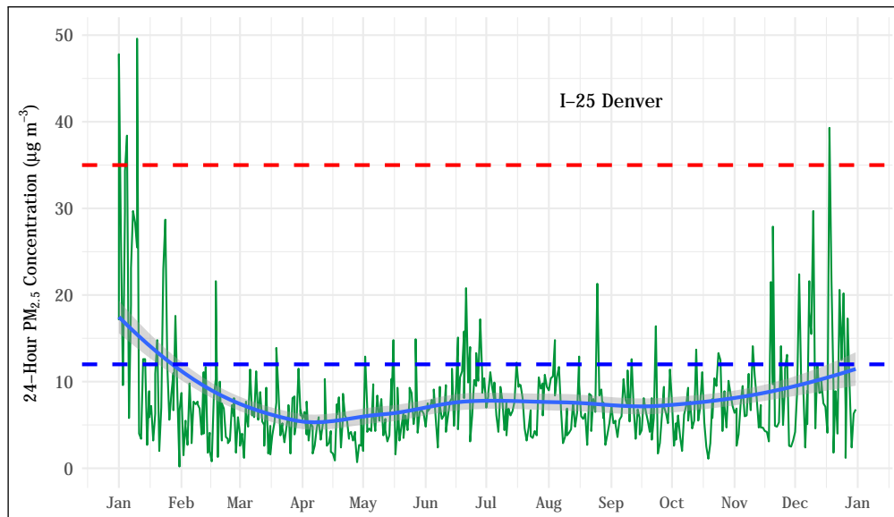
Figure 5.64: 24-hour average PM_{2.5} concentrations at the I-25 Denver station. The mean trend obtained using a generalized additive model is shown as a blue line. The 24-hour standard ( 35 \mu\text{g m}^{-3} ) is shown as a dashed red line. The annual mean standard ( 12 \mu\text{g m}^{-3} ) is shown as a dashed blue line. The exceedances which took place in January and December have been flagged by the division as exceptional prolonged inversion events.
