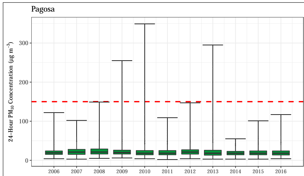
Figure 4.67: 24-hour average PM 10 concentrations at the Pagosa Springs School station. The 24-hour standard (150 µg m -3 ) is shown as a dashed red line.
