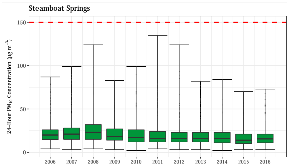
Figure 4.4: 24-hr PM 10 concentrations at the Steamboat Springs station. The 24-hour standard (150 µg m -3 ) is shown as a dashed red line.
