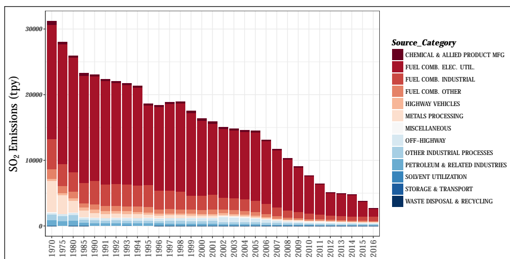
Figure 2.5: Trends in national sulfur dioxide emissions from 1970 to 2016.
