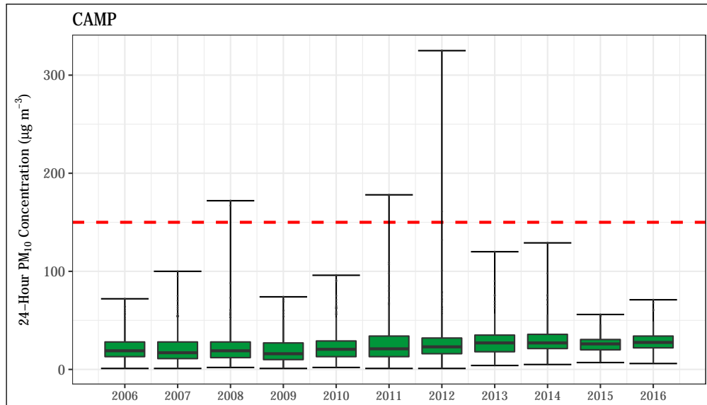
Figure 4.11: 24-hr PM 10 concentrations at the CAMP station. The 24-hour standard (150 µg m -3 ) is shown as a dashed red line.
