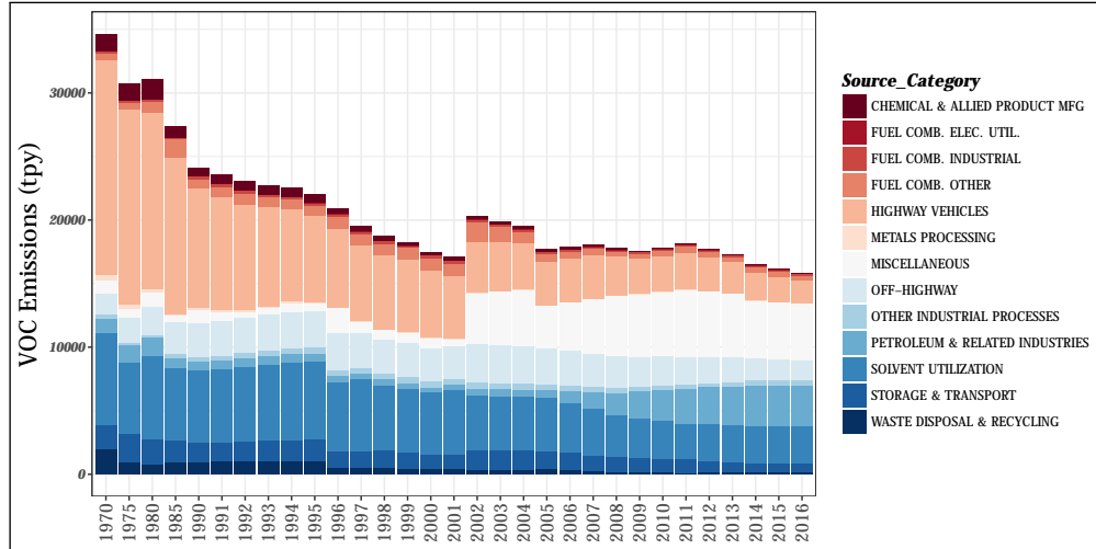
Figure 2.8: Trends in national VOC emissions from 1970 to 2016.
