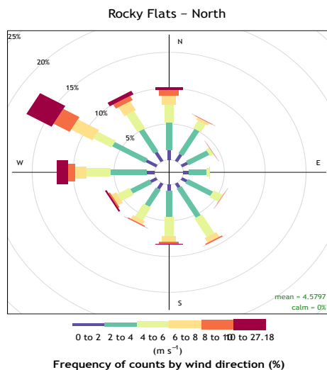
Figure 4.53: Wind roses for sites in the Denver Metro/North Front Range Region during 2016 (continued).
