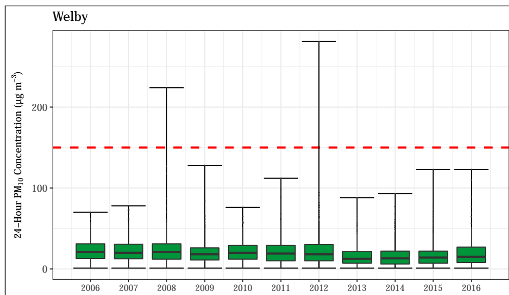
Figure 4.5: 24-hr PM 10 concentrations at the Welby station. The 24-hour standard (150 µg m -3 ) is shown as a dashed red line.
