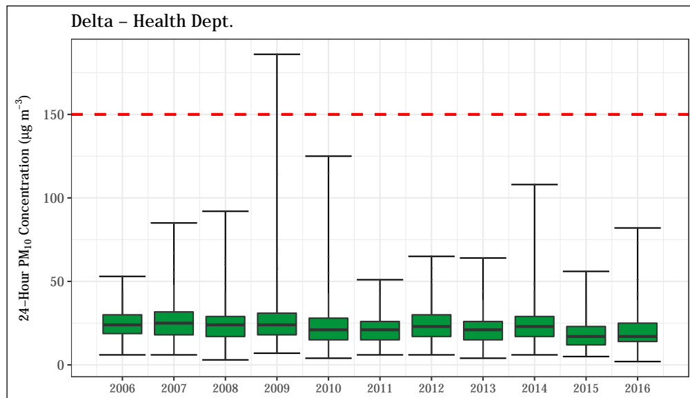
Figure 4.70: 24-hour average PM 10 concentrations at the Delta - Health Dept. station. The 24-hour standard (150 µg m -3 ) is shown as a dashed red line.
