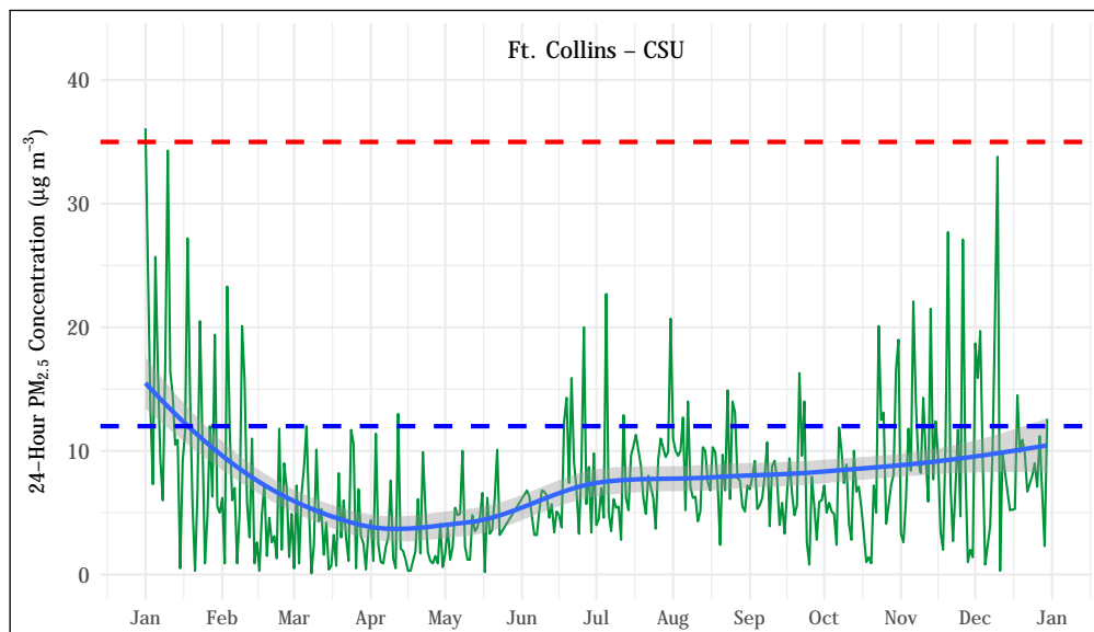
Figure 5.69: 24-hour average PM_{2.5} concentrations at the Ft. Collins - CSU GRIMM station. The mean trend obtained using a generalized additive model is shown as a blue line. The 24-hour standard ( 35 \mu\text{g m}^{-3} ) is shown as a dashed red line. The annual mean standard ( 12 \mu\text{g m}^{-3} ) is shown as a dashed blue line. The low volume particulate sampler was removed as of July, 2016, so PM_{2.5} is now recorded by use of a GRIMM continuous particulate monitor which has been in operation since June 2015. The spike in January has been flagged by the division as exceptional prolonged inversion event.
