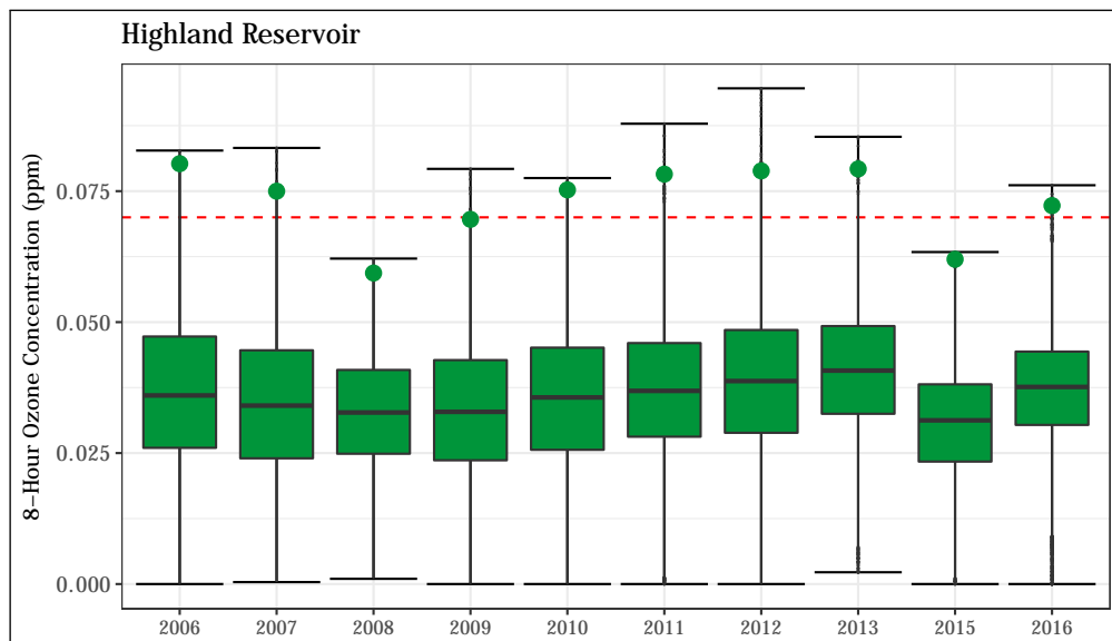
Figure 4.31: 8-hour average O 3 concentrations at the Highlands station. The 8-hour standard (0.070 ppm) is shown as a dashed red line. The annual design value (4 th highest daily maximum 8-hour average value) is shown for each year as a green point.
