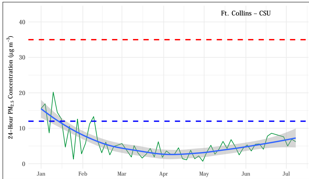
Figure 5.68: 24-hour average PM_{2.5} concentrations at the Ft. Collins - CSU station. The mean trend obtained using a generalized additive model is shown as a blue line. The 24-hour standard ( 35 \mu\text{g m}^{-3} ) is shown as a dashed red line. The annual mean standard ( 12 \mu\text{g m}^{-3} ) is shown as a dashed blue line. The low volume particulate sampler was removed as of July, 2016, so PM_{2.5} is now recorded by use of a GRIMM continuous particulate monitor which has been in operation since June 2015.
