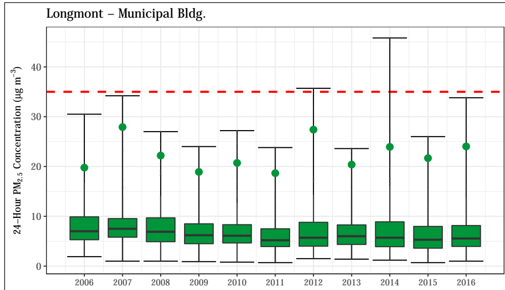
Figure 4.8: 24-hr PM 2.5 concentrations at the Longmont - Municipal Bldg. station. The 24-hour standard (35 µg m -3 ) is shown as a dashed red line. The annual design value (98 th percentile of values measured throughout the year) is shown for each year as a green point.
