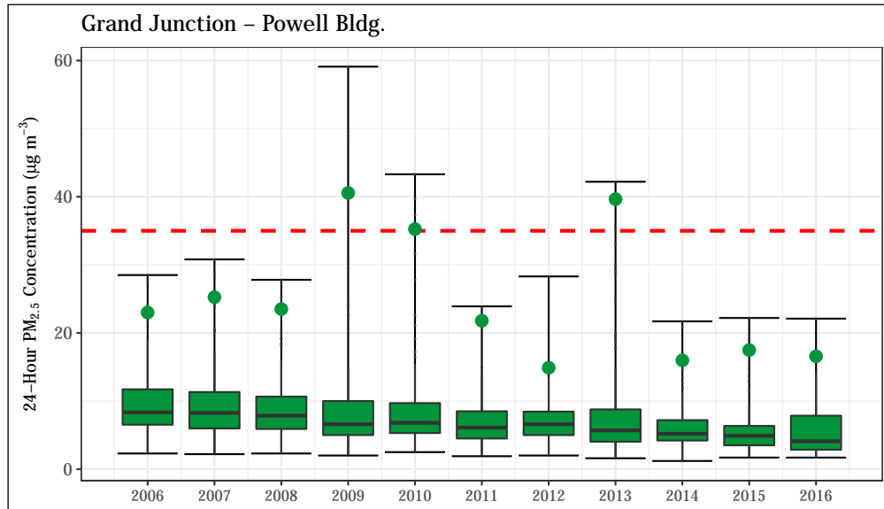
Figure 4.75: 24-hr PM 2.5 concentrations at the Grand Junction - Powell Bldg. station. The 24-hour standard (35 µg m -3 ) is shown as a dashed red line. The annual design value (98 th percentile of values measured throughout the year) is shown for each year as a green point.
