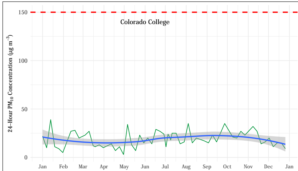
Figure 5.44: 24-hour average PM_{10} concentrations at the Colorado College station. The mean trend obtained using a generalized additive model is shown as a blue line. The 24-hour standard ( 150 \mu\text{g m}^{-3} ) is shown as a dashed red line.
