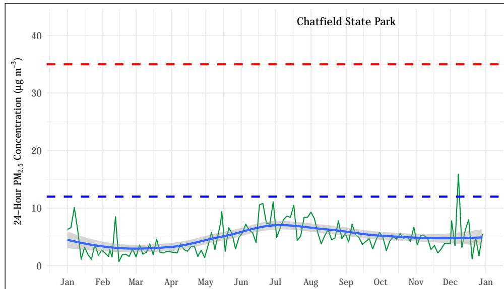
Figure 5.66: 24-hour average PM_{2.5} concentrations at the Chatfield State Park station. The mean trend obtained using a generalized additive model is shown as a blue line. The 24-hour standard ( 35 \mu\text{g m}^{-3} ) is shown as a dashed red line. The annual mean standard ( 12 \mu\text{g m}^{-3} ) is shown as a dashed blue line.
