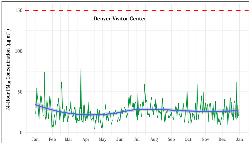
Figure 5.42: 24-hour average PM_{10} concentrations at the Denver Visitor Center station. The mean trend obtained using a generalized additive model is shown as a blue line. The 24-hour standard ( 150 \mu\text{g m}^{-3} ) is shown as a dashed red line.
