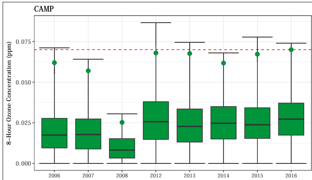
Figure 4.34: 8-hour average O 3 concentrations at the CAMP station. The 8-hour standard (0.070 ppm) is shown as a dashed red line. The annual design value (4 th highest daily maximum 8-hour average value) is shown for each year as a green point.
