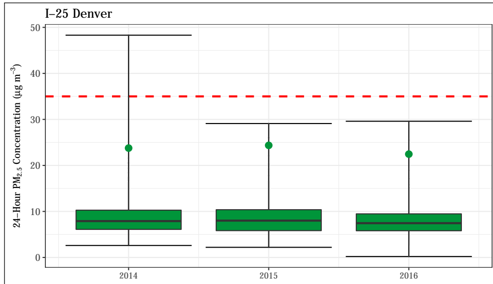
Figure 4.16: 24-hr PM 2.5 concentrations at the I-25 Denver station. The 24-hour standard (35 µg m -3 ) is shown as a dashed red line. The annual design value (98 th percentile of values measured throughout the year) is shown for each year as a green point.
