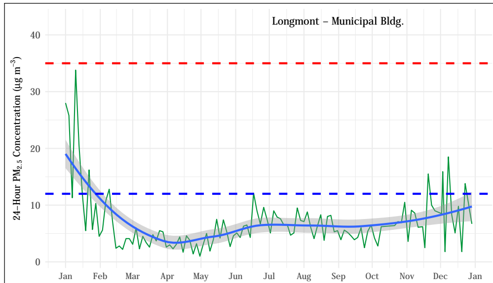
Figure 5.60: 24-hour average PM_{2.5} concentrations at the Longmont - Municipal Bldg. station. The mean trend obtained using a generalized additive model is shown as a blue line. The 24-hour standard ( 35 \mu\text{g m}^{-3} ) is shown as a dashed red line. The annual mean standard ( 12 \mu\text{g m}^{-3} ) is shown as a dashed blue line.
