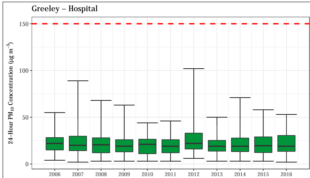
Figure 4.21: 24-hr PM 10 concentrations at the Greeley - Hospital station. The 24-hour standard (150 µg m -3 ) is shown as a dashed red line.
