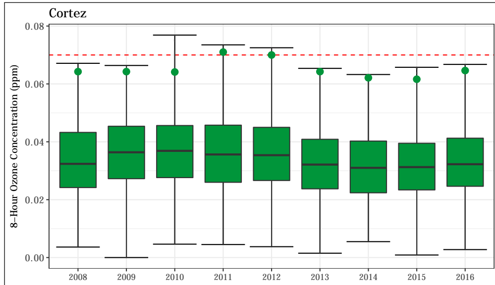
Figure 4.69: 8-hour average O 3 concentrations at the Cortez - Health Dept. station. The 8-hour standard (0.070 ppm) is shown as a dashed red line. The annual design value (4 th highest daily maximum 8-hour average value) is shown for each year as a green point.
