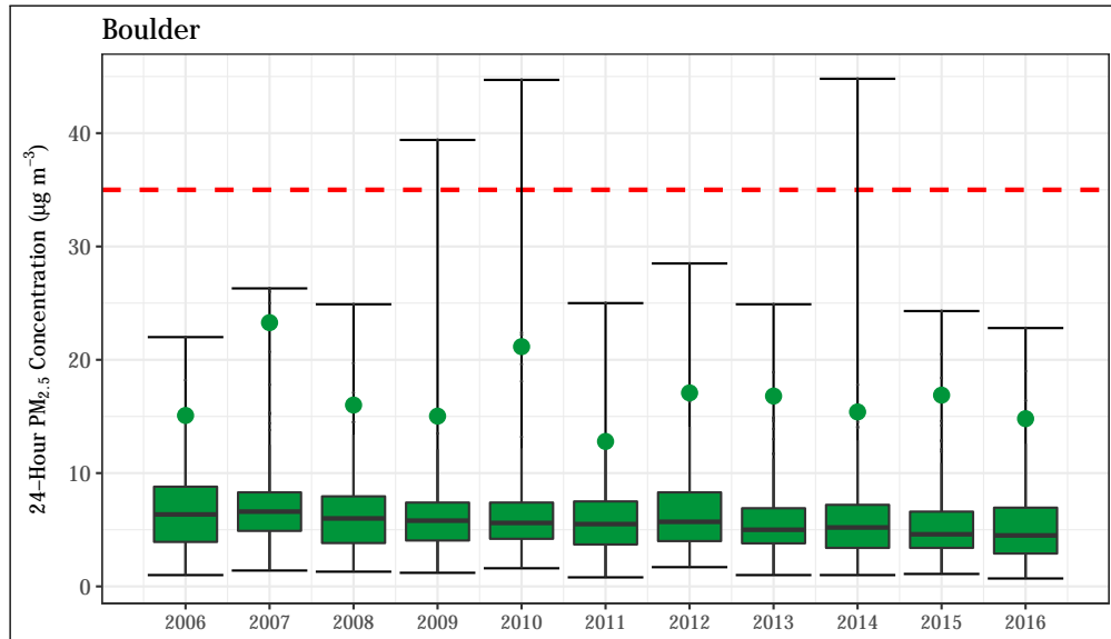
Figure 4.10: 24-hr PM 2.5 concentrations at the Boulder Chamber of Commerce station. The 24-hour standard (35 µg m -3 ) is shown as a dashed red line. The annual design value (98 th percentile of values measured throughout the year) is shown for each year as a green point.
