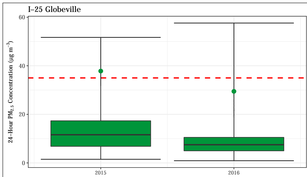
Figure 4.17: 24-hr PM 2.5 concentrations at the I-25 Globeville GRIMM station. The 24-hour standard (35 µg m -3 ) is shown as a dashed red line. The annual design value (98 th percentile of values measured throughout the year) is shown for each year as a green point. The Globeville station has only been in operation since October, 2015, so the 2015 data only represents three months of data.
