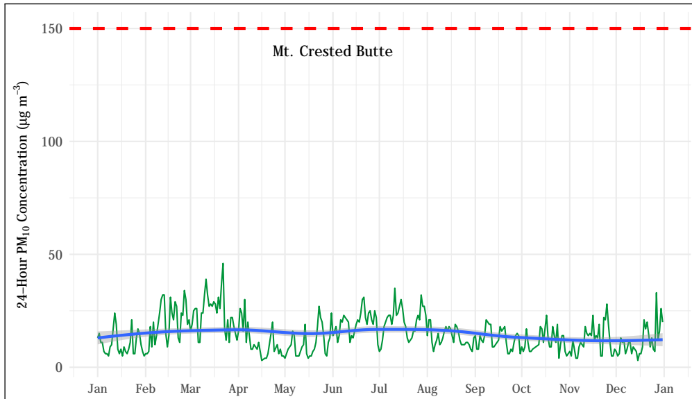
Figure 5.50: 24-hour average PM_{10} concentrations at the Mt. Crested Butte station. The mean trend obtained using a generalized additive model is shown as a blue line. The 24-hour standard ( 150 \mu\text{g m}^{-3} ) is shown as a dashed red line.
