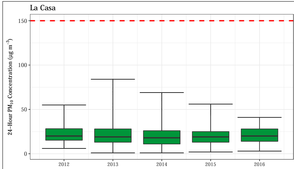
Figure 4.14: 24-hr PM 10 concentrations at the La Casa station. The 24-hour standard (150 µg m -3 ) is shown as a dashed red line.
