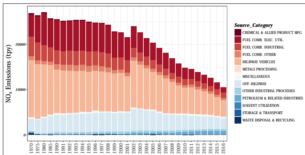
Figure 2.11: Trends in national NO x emissions from 1970 to 2016.
