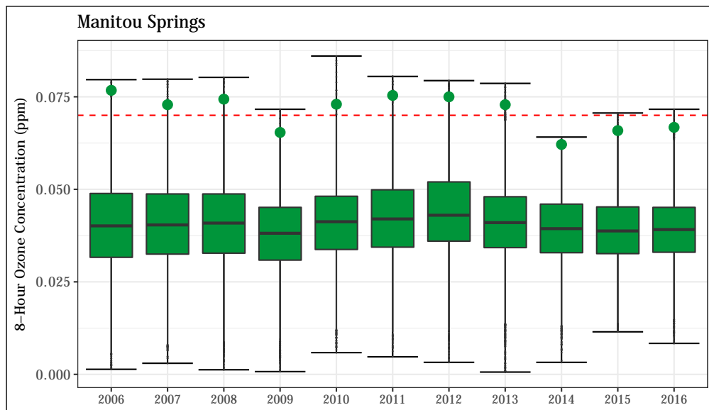
Figure 4.60: 8-hour average O 3 concentrations at the Manitou Springs station. The 8-hour standard (0.070 ppm) is shown as a dashed red line. The annual design value (4 th highest daily maximum 8-hour average value) is shown for each year as a green point.
