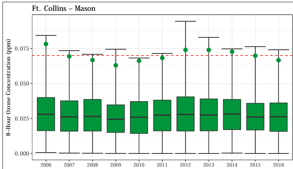
Figure 4.42: 8-hour average O 3 concentrations at the Ft. Collins - Mason station. The 8-hour standard (0.070 ppm) is shown as a dashed red line. The annual design value (4 th highest daily maximum 8-hour average value) is shown for each year as a green point.
