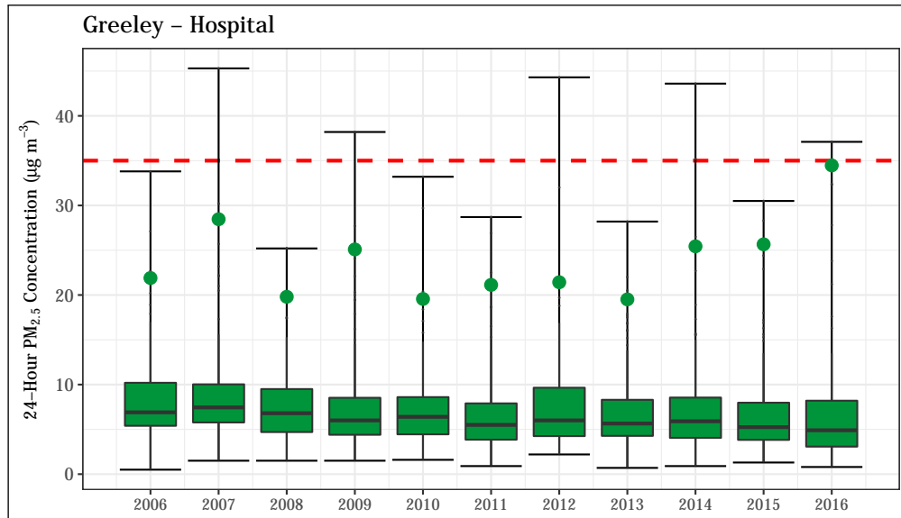
Figure 4.22: 24-hr PM 2.5 concentrations at the Greeley - Hospital station. The 24-hour standard (35 µg m -3 ) is shown as a dashed red line. The annual design value (98 th percentile of values measured throughout the year) is shown for each year as a green point.
