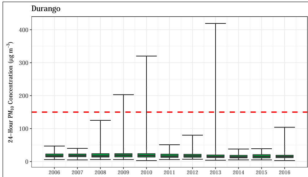
Figure 4.68: 24-hour average PM 10 concentrations at the Durango station. The 24-hour standard (150 µg m -3 ) is shown as a dashed red line.
