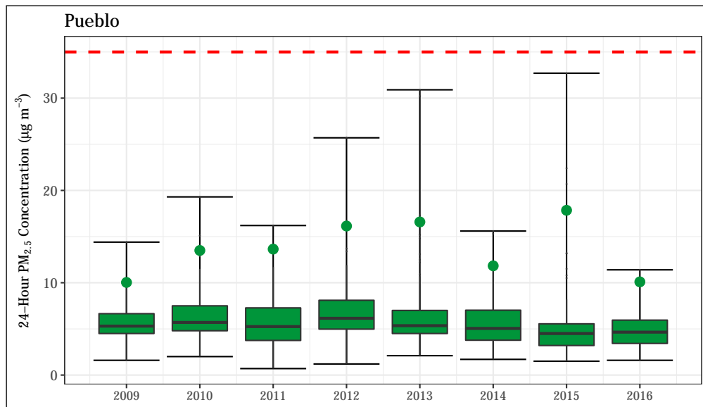
Figure 4.66: 24-hr PM 2.5 concentrations at the Pueblo station. The 24-hour standard (35 µg m -3 ) is shown as a dashed red line. The annual design value (98 th percentile of values measured throughout the year) is shown for each year as a green point.
