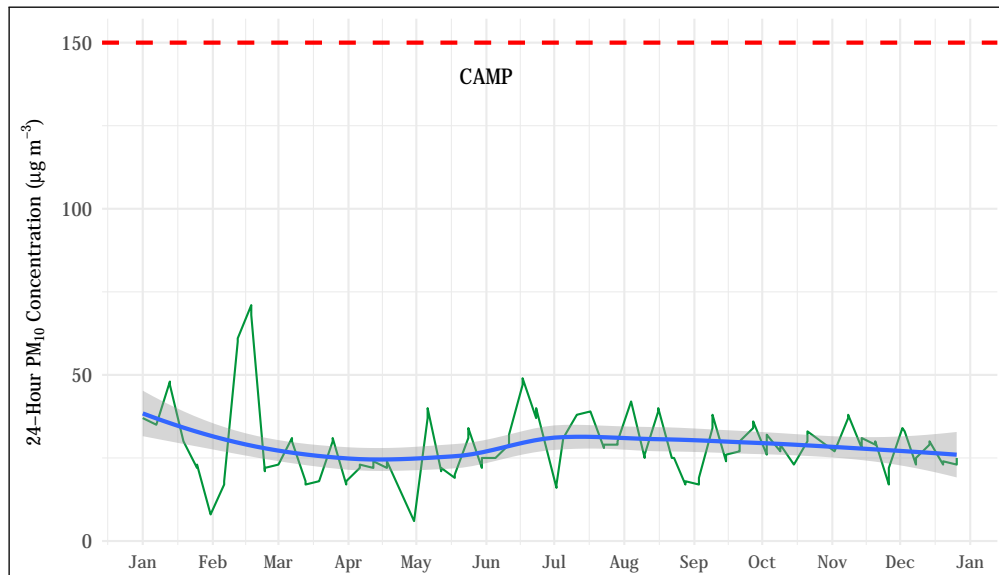
Figure 5.41: 24-hour average PM_{10} concentrations at the CAMP station. The mean trend obtained using a generalized additive model is shown as a blue line. The 24-hour standard ( 150 \mu\text{g m}^{-3} ) is shown as a dashed red line.
