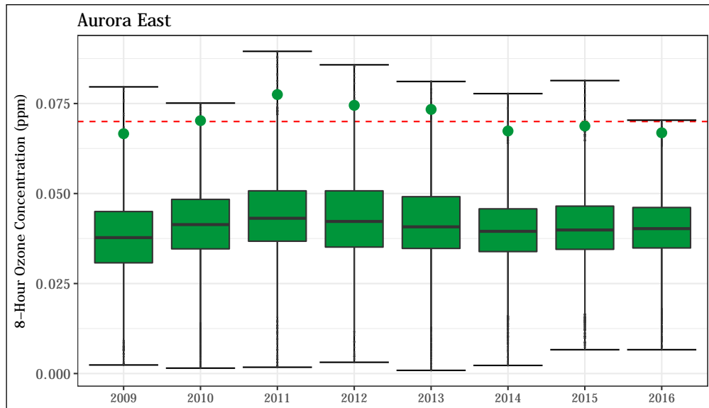
Figure 4.32: 8-hour average O 3 concentrations at the Aurora - East station. The 8-hour standard (0.070 ppm) is shown as a dashed red line. The annual design value (4 th highest daily maximum 8-hour average value) is shown for each year as a green point.
