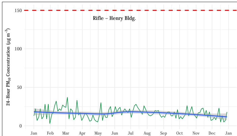
Figure 5.47: 24-hour average PM_{10} concentrations at the Rifle - Henry Bldg. station. The mean trend obtained using a generalized additive model is shown as a blue line. The 24-hour standard ( 150 \mu\text{g m}^{-3} ) is shown as a dashed red line.
