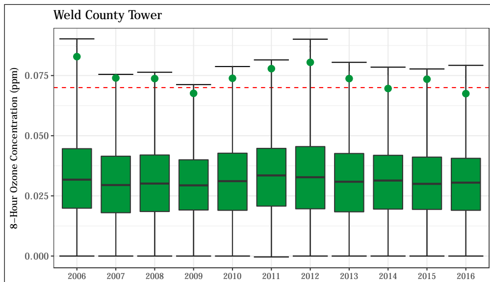
Figure 4.43: 8-hour average O 3 concentrations at the Greeley - County Tower station. The 8-hour standard (0.070 ppm) is shown as a dashed red line. The annual design value (4 th highest daily maximum 8-hour average value) is shown for each year as a green point.
