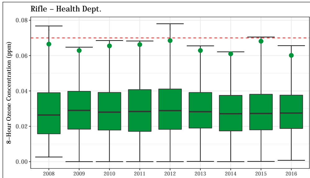
Figure 4.79: 8-hour average O 3 concentrations at the Rifle - Health Dept. station. The 8-hour standard (0.070 ppm) is shown as a dashed red line. The annual design value (4 th highest daily maximum 8-hour average value) is shown for each year as a green point.
