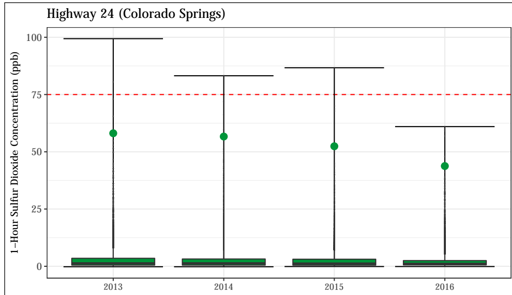
Figure 4.61: 1-hour average SO 2 concentrations at the Highway 24 station. The annual design value (99 th percentile of daily maximum 1-hour values) is shown for each year as a green point.
