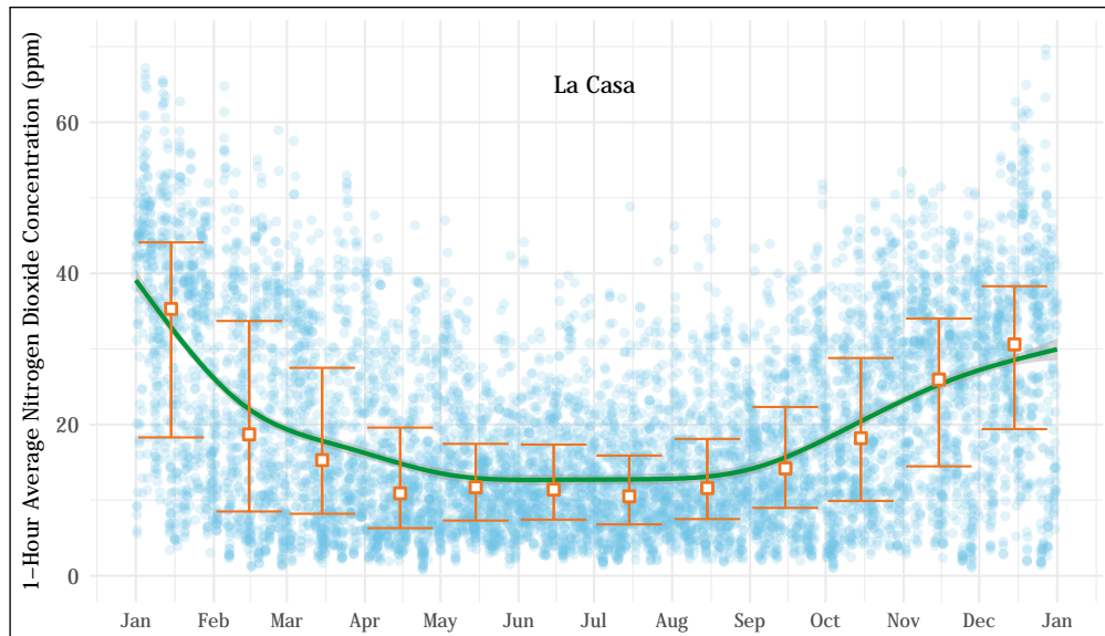
Figure 5.33: 1-hour average NO 2 concentrations at the La Casa station (blue dots). The mean trend obtained using a generalized additive model is shown as a green line. The error bars represent the median and interquartile range of values observed during each month.
