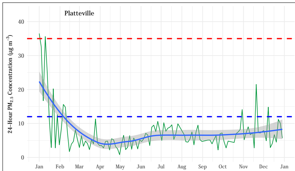
Figure 5.74: 24-hour average PM_{2.5} concentrations at the Platteville station. The mean trend obtained using a generalized additive model is shown as a blue line. The 24-hour standard ( 35 \mu\text{g m}^{-3} ) is shown as a dashed red line. The annual mean standard ( 12 \mu\text{g m}^{-3} ) is shown as a dashed blue line.
