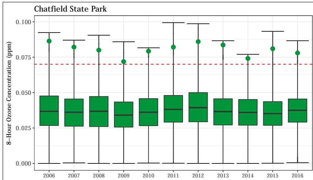
Figure 4.36: 8-hour average O 3 concentrations at the Chatfield State Park station. The 8-hour standard (0.070 ppm) is shown as a dashed red line. The annual design value (4 th highest daily maximum 8-hour average value) is shown for each year as a green point.
