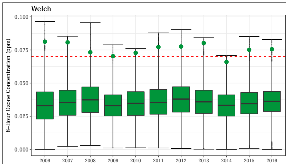
Figure 4.37: 8-hour average O 3 concentrations at the Welch station. The 8-hour standard (0.070 ppm) is shown as a dashed red line. The annual design value (4 th highest daily maximum 8-hour average value) is shown for each year as a green point.
