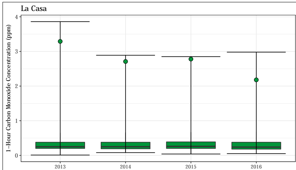
Figure 4.26: 1-hour average CO concentrations at the La Casa station. The annual design value (2 nd highest 1-hour value) is shown for each year as a green point.
