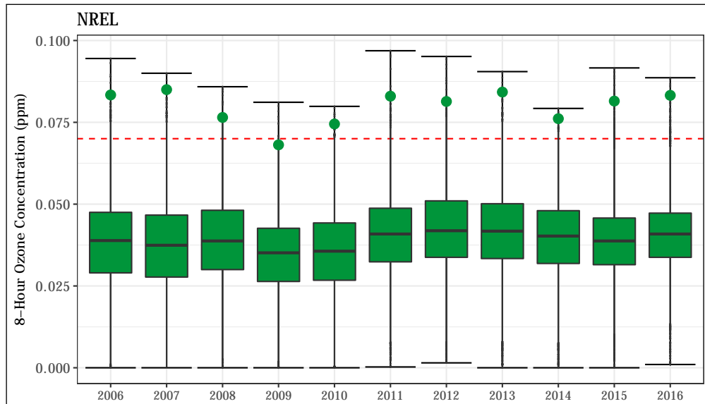
Figure 4.39: 8-hour average O 3 concentrations at the NREL station. The 8-hour standard (0.070 ppm) is shown as a dashed red line. The annual design value (4 th highest daily maximum 8-hour average value) is shown for each year as a green point.
