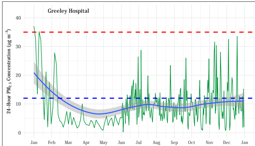
Figure 5.73: 24-hour average PM_{2.5} concentrations at the Greeley - Hospital station. The mean trend obtained using a generalized additive model is shown as a blue line. The 24-hour standard ( 35 \mu\text{g m}^{-3} ) is shown as a dashed red line. The annual mean standard ( 12 \mu\text{g m}^{-3} ) is shown as a dashed blue line.
