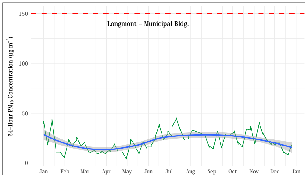
Figure 5.39: 24-hour average PM_{10} concentrations at the Longmont - Municipal Bldg. station. The mean trend obtained using a generalized additive model is shown as a blue line. The 24-hour standard ( 150 \mu\text{g m}^{-3} ) is shown as a dashed red line.
