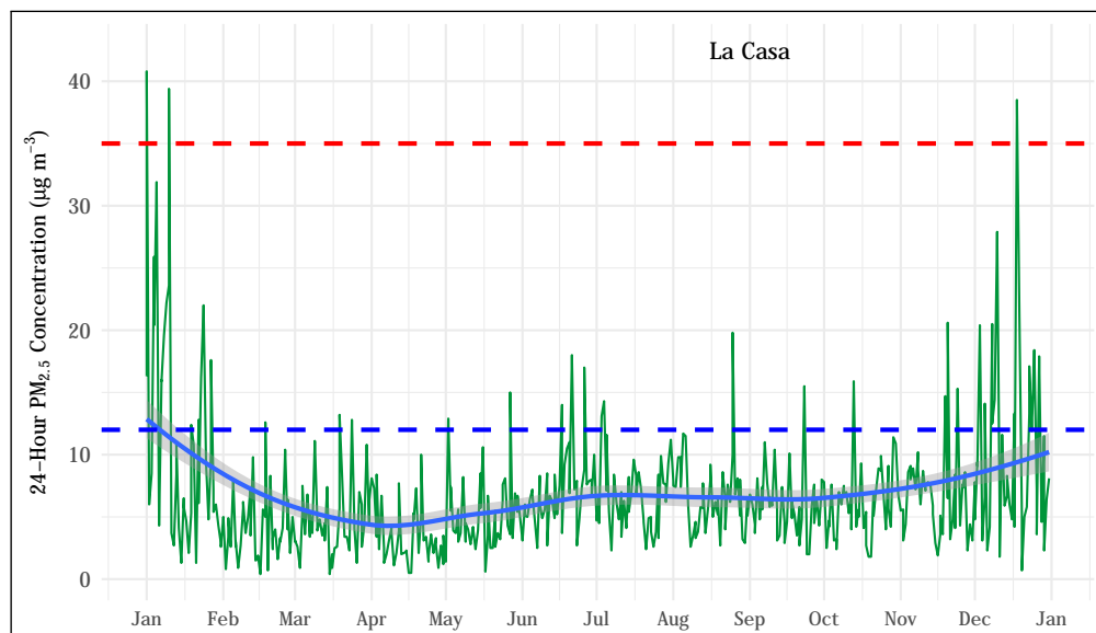
Figure 5.63: 24-hour average PM_{2.5} concentrations at the La Casa station. The mean trend obtained using a generalized additive model is shown as a blue line. The 24-hour standard ( 35 \mu\text{g m}^{-3} ) is shown as a dashed red line. The annual mean standard ( 12 \mu\text{g m}^{-3} ) is shown as a dashed blue line. The exceedances which took place in January and December have been flagged by the division as exceptional prolonged inversion events.
