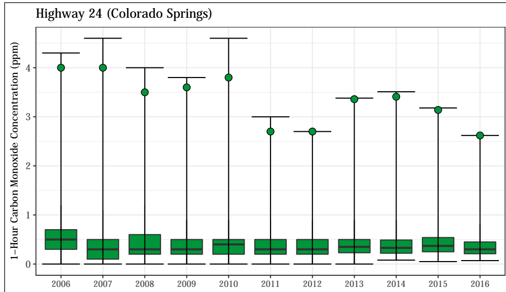
Figure 4.58: 1-hour average CO concentrations at the Highway 24 station. The annual design value (2 nd highest 1-hour value) is shown for each year as a green point.
