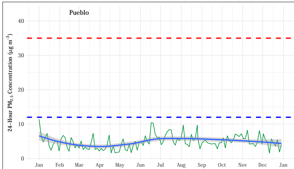
Figure 5.72: 24-hour average PM_{2.5} concentrations at the Pueblo station. The mean trend obtained using a generalized additive model is shown as a blue line. The 24-hour standard ( 35 \mu\text{g m}^{-3} ) is shown as a dashed red line. The annual mean standard ( 12 \mu\text{g m}^{-3} ) is shown as a dashed blue line.
