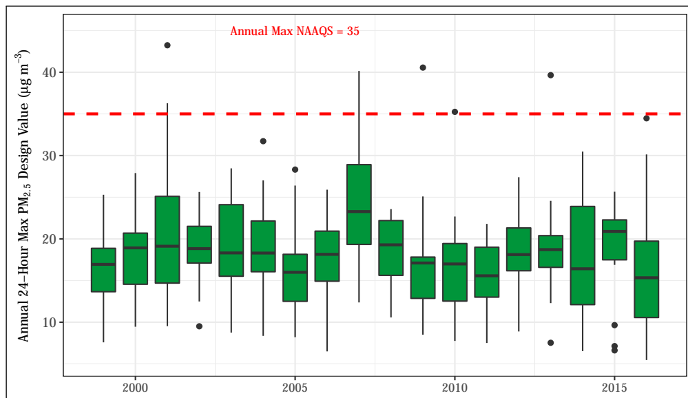
Figure 2.19: Statewide historical record of 24-hour maximum PM 2.5 design values. The box plot shows the mean design value statewide for each year, as well as the interquartile range (box) of values observed at monitoring sites throughout the state and the minimum and maximum values. Outliers are indicated by black points.
