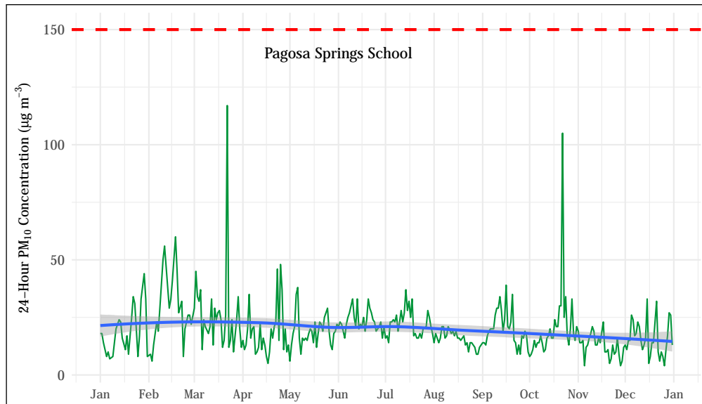
Figure 5.38: 24-hour average PM_{10} concentrations at the Pagosa Springs School station. The mean trend obtained using a generalized additive model is shown as a blue line. The 24-hour standard ( 150 \mu\text{g m}^{-3} ) is shown as a dashed red line.
