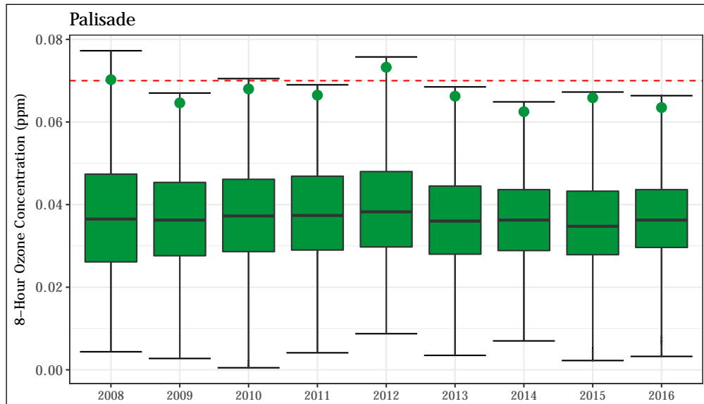
Figure 4.80: 8-hour average O 3 concentrations at the Palisade station. The 8-hour standard (0.070 ppm) is shown as a dashed red line. The annual design value (4 th highest daily maximum 8-hour average value) is shown for each year as a green point.
