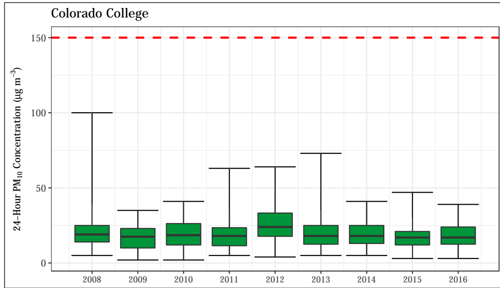
Figure 4.57: 24-hour average PM 10 concentrations at the Colorado College station. The 24-hour standard (150 µg m -3 ) is shown as a dashed red line.
