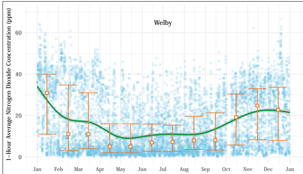
Figure 5.31: 1-hour average NO 2 concentrations at the Welby station (blue dots). The mean trend obtained using a generalized additive model is shown as a green line. The error bars represent the median and interquartile range of values observed during each month.
