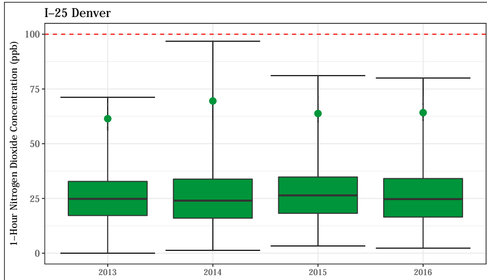
Figure 4.47: 1-hour average NO 2 concentrations at the I-25 Denver station. The annual design value (98 th percentile of daily maximum 1-hour values) is shown for each year as a green point.
