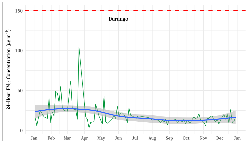
Figure 5.51: 24-hour average PM_{10} concentrations at the Durango station. The mean trend obtained using a generalized additive model is shown as a blue line. The 24-hour standard ( 150 \mu\text{g m}^{-3} ) is shown as a dashed red line.
