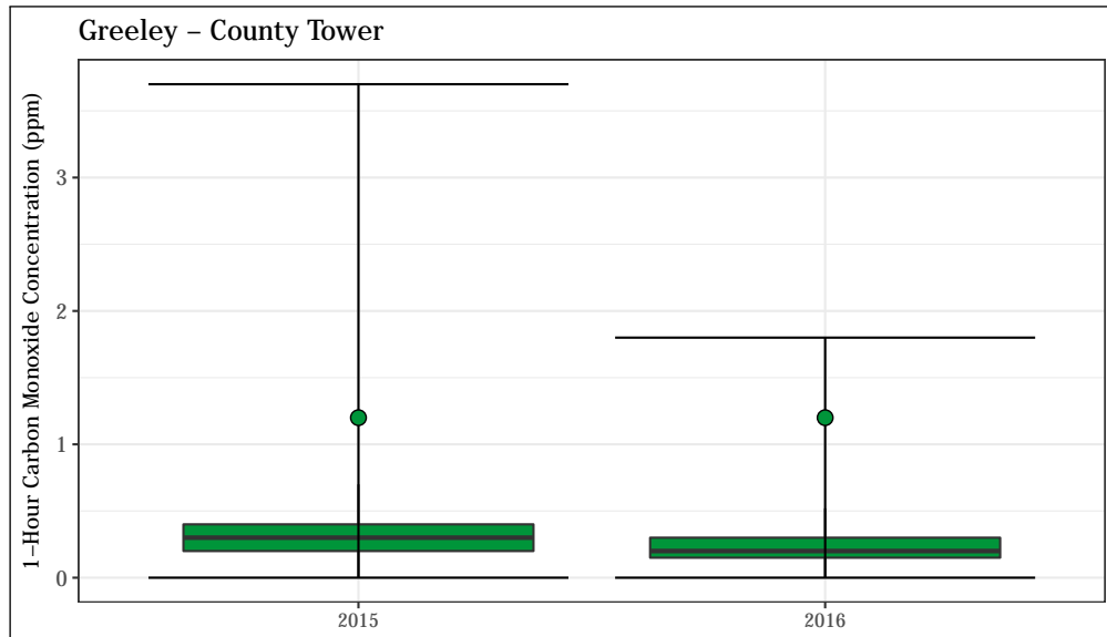
Figure 4.29: 1-hour average CO concentrations at the Greeley - County Tower station. The annual design value (2 nd highest 1-hour value) is shown for each year as a green point.
