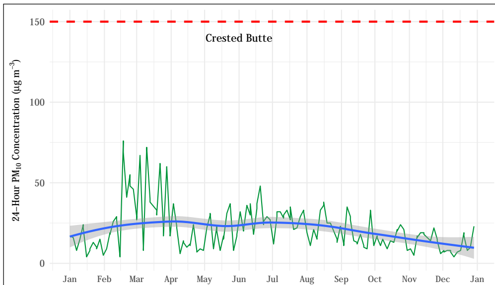
Figure 5.49: 24-hour average PM_{10} concentrations at the Crested Butte station. The mean trend obtained using a generalized additive model is shown as a blue line. The 24-hour standard ( 150 \mu\text{g m}^{-3} ) is shown as a dashed red line.
