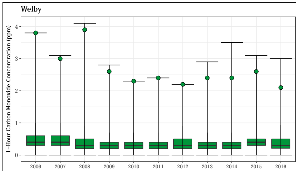
Figure 4.24: 1-hour average CO concentrations at the Welby station. The annual design value (2 nd highest 1-hour value) is shown for each year as a green point.
