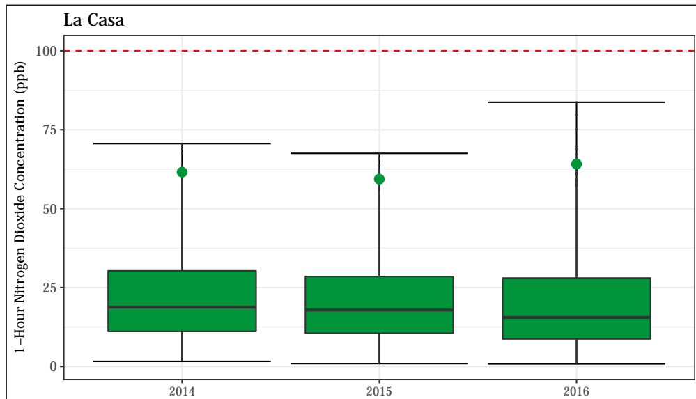
Figure 4.46: 1-hour average NO 2 concentrations at the La Casa station. The annual design value (98 th percentile of daily maximum 1-hour values) is shown for each year as a green point.
