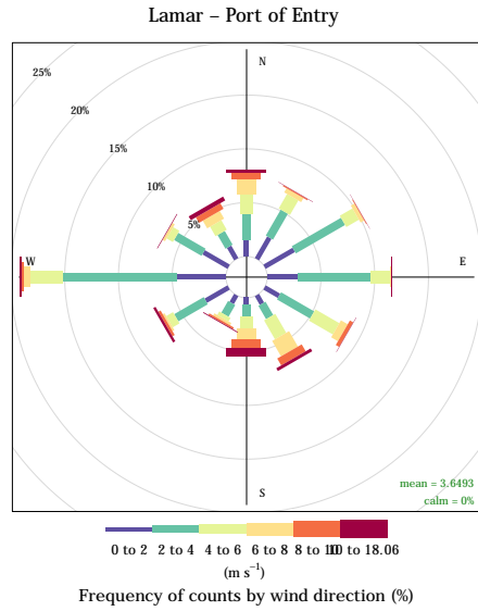
Figure 4.56: Wind rose from the Lamar - Port of Entry meteorological station.
