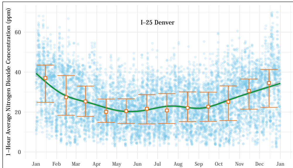
Figure 5.34: 1-hour average NO 2 concentrations at the I-25 Denver station (blue dots). The mean trend obtained using a generalized additive model is shown as a green line. The error bars represent the median and interquartile range of values observed during each month.
