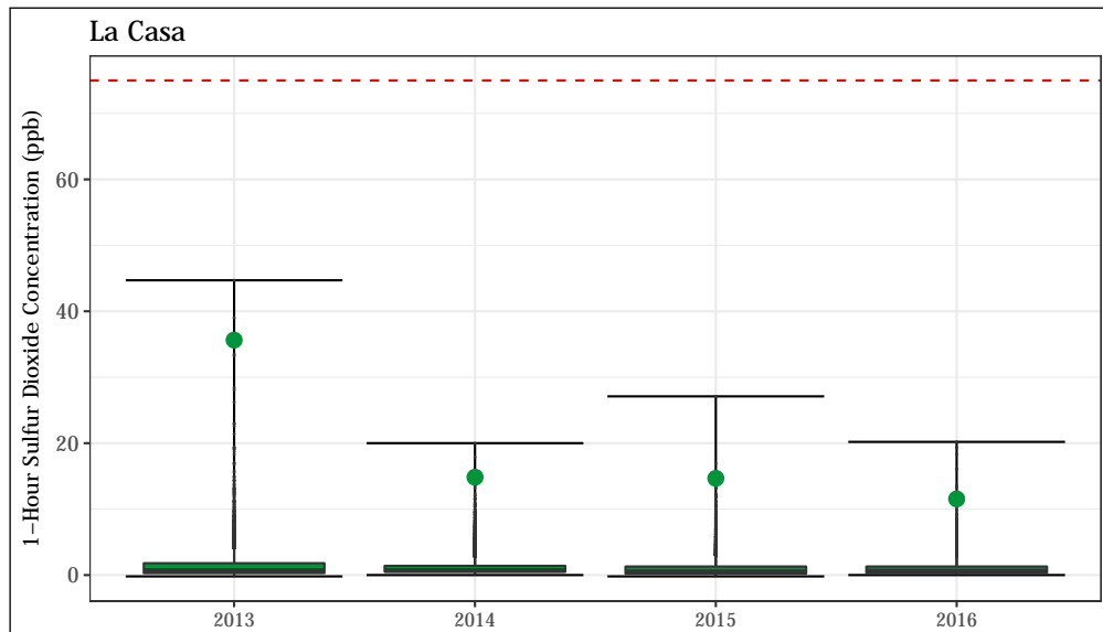
Figure 4.51: 1-hour average SO 2 concentrations at the La Casa station. The annual design value (99 th percentile of daily maximum 1-hour values) is shown for each year as a green point.
