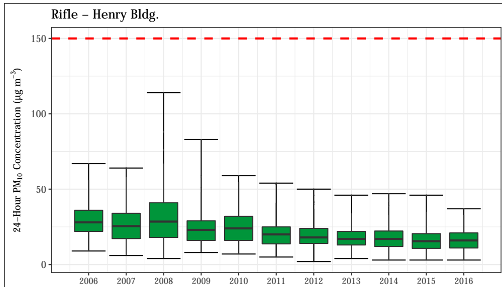
Figure 4.72: 24-hour average PM 10 concentrations at the Rifle - Henry Bldg. station. The 24-hour standard (150 µg m -3 ) is shown as a dashed red line.
