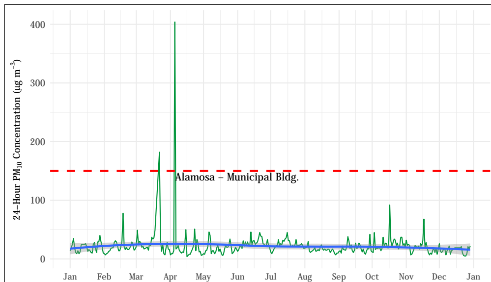
Figure 5.37: 24-hour average PM_{10} concentrations at the Alamosa - Municipal Bldg. station. The mean trend obtained using a generalized additive model is shown as a blue line. The 24-hour standard ( 150 \mu\text{g m}^{-3} ) is shown as a dashed red line. The two exceedances which took place on March 22 nd and April 5 th have been flagged by the division as exceptional high wind events.
