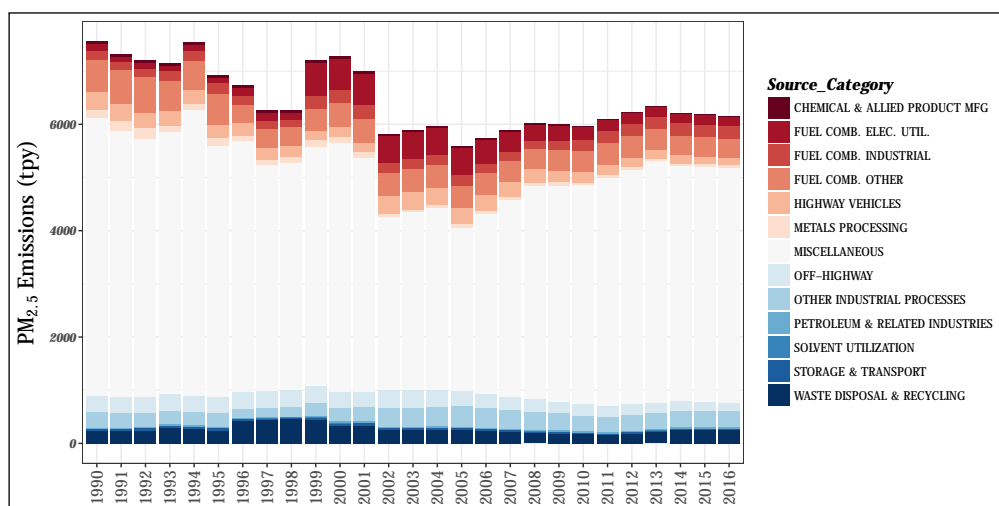
Figure 2.16: Trends in national PM 2.5 emissions from 1990 to 2016.
