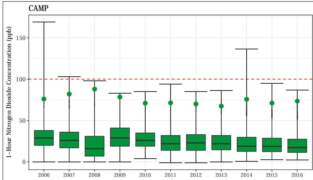
Figure 4.45: 1-hour average NO 2 concentrations at the CAMP station. The annual design value (98 th percentile of daily maximum 1-hour values) is shown for each year as a green point.
