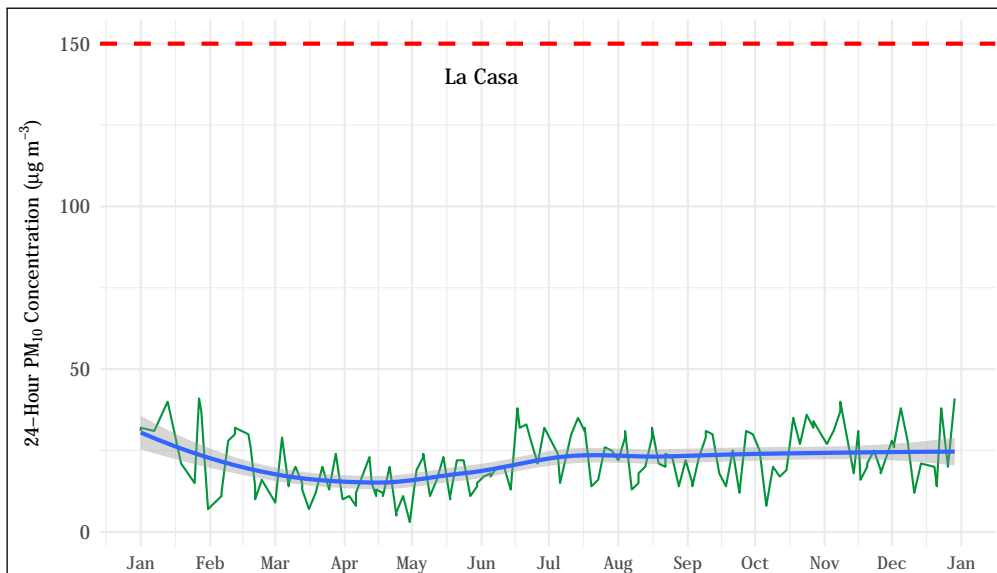
Figure 5.43: 24-hour average PM_{10} concentrations at the La Casa station. The mean trend obtained using a generalized additive model is shown as a blue line. The 24-hour standard ( 150 \mu\text{g m}^{-3} ) is shown as a dashed red line.
