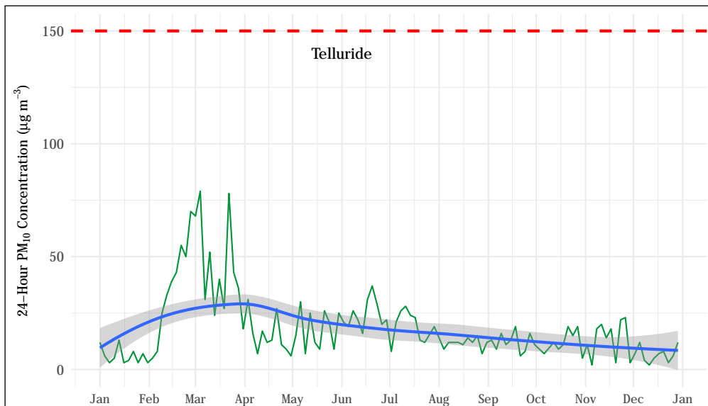
Figure 5.57: 24-hour average PM_{10} concentrations at the Telluride station. The mean trend obtained using a generalized additive model is shown as a blue line. The 24-hour standard ( 150 \mu\text{g m}^{-3} ) is shown as a dashed red line.
