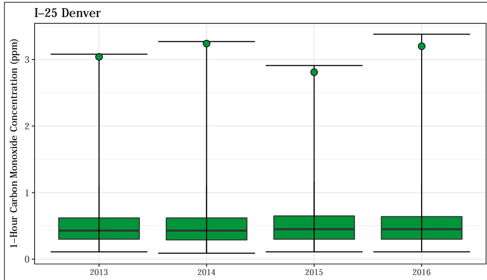
Figure 4.27: 1-hour average CO concentrations at the I-25 Denver station. The annual design value (2 nd highest 1-hour value) is shown for each year as a green point.
