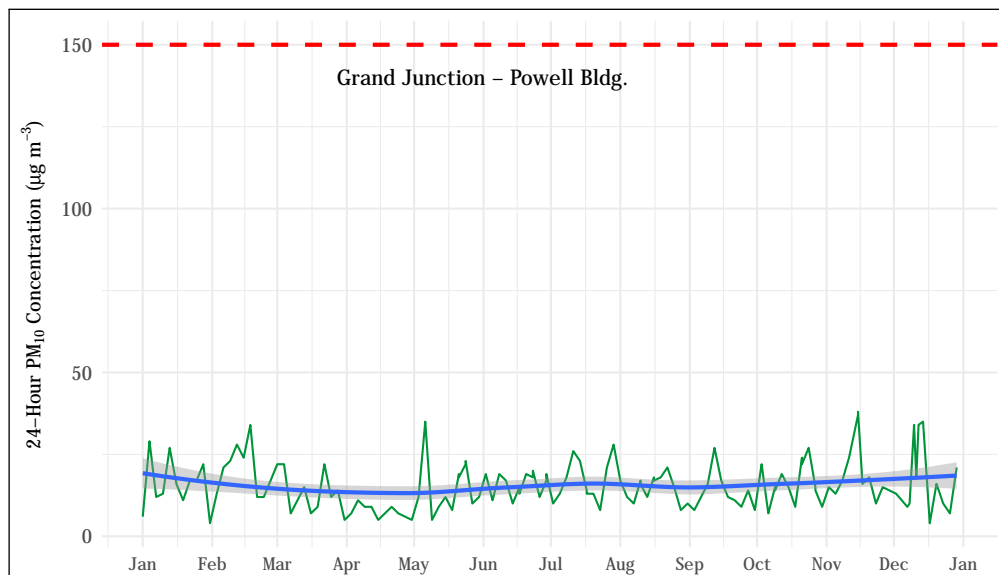
Figure 5.53: 24-hour average PM_{10} concentrations at the Grand Junction - Powell station. The mean trend obtained using a generalized additive model is shown as a blue line. The 24-hour standard ( 150 \mu\text{g m}^{-3} ) is shown as a dashed red line.
