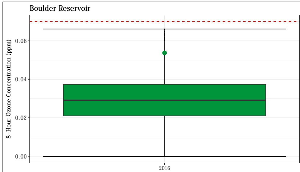
Figure 4.33: 8-hour average O 3 concentrations at the Boulder Reservoir station. The 8-hour standard (0.070 ppm) is shown as a dashed red line. The annual design value (4 th highest daily maximum 8-hour average value) is shown for each year as a green point.
