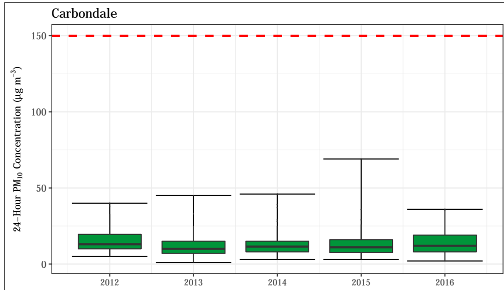
Figure 4.73: 24-hour average PM 10 concentrations at the Carbondale station. The 24-hour standard (150 µg m -3 ) is shown as a dashed red line.
