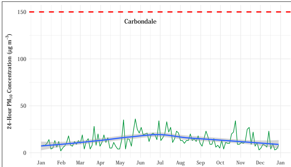
Figure 5.48: 24-hour average PM_{10} concentrations at the Carbondale station. The mean trend obtained using a generalized additive model is shown as a blue line. The 24-hour standard ( 150 \mu\text{g m}^{-3} ) is shown as a dashed red line.
