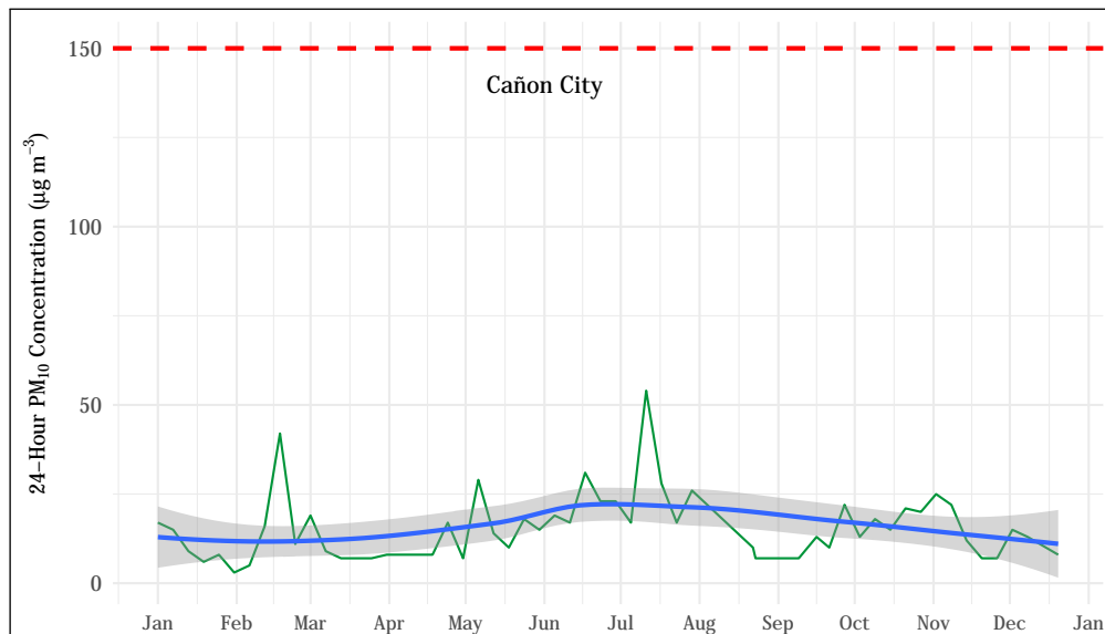
Figure 5.45: 24-hour average PM_{10} concentrations at the Cañon City station. The mean trend obtained using a generalized additive model is shown as a blue line. The 24-hour standard ( 150 \mu\text{g m}^{-3} ) is shown as a dashed red line.
