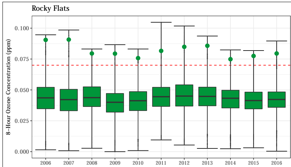
Figure 4.38: 8-hour average O 3 concentrations at the Rocky Flats - N. station. The 8-hour standard (0.070 ppm) is shown as a dashed red line. The annual design value (4 th highest daily maximum 8-hour average value) is shown for each year as a green point.
