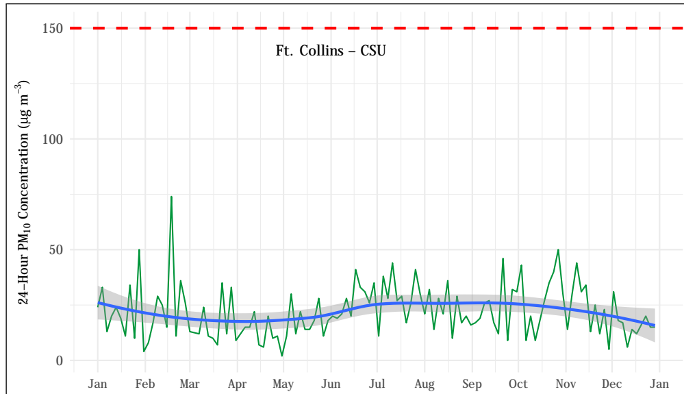
Figure 5.52: 24-hour average PM_{10} concentrations at the Ft. Collins - CSU station. The mean trend obtained using a generalized additive model is shown as a blue line. The 24-hour standard ( 150 \mu\text{g m}^{-3} ) is shown as a dashed red line.
