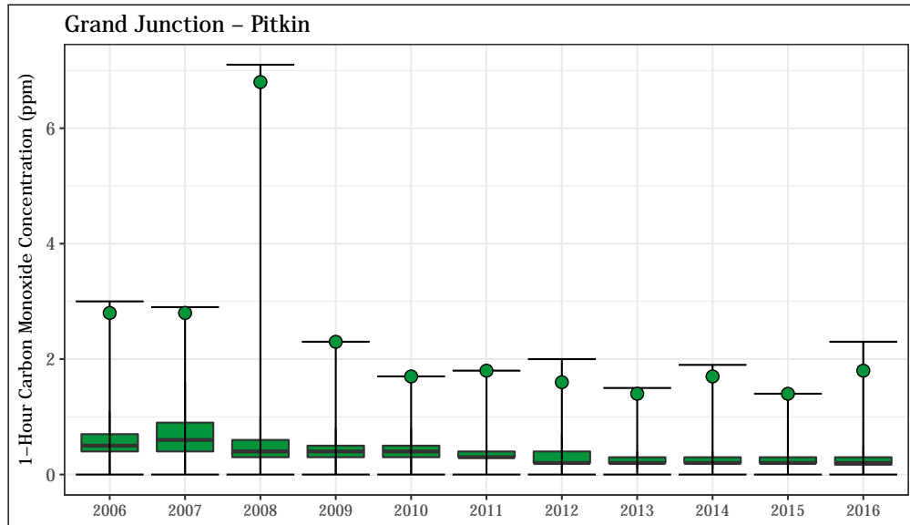
Figure 4.77: 1-hour average CO concentrations at the Grand Junction - Pitkin station. The annual design value (2 nd highest 1-hour value) is shown for each year as a green point.
