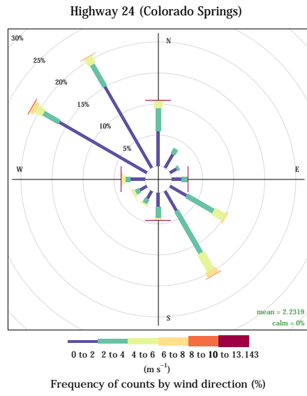
Figure 4.62: Wind rose from the Highway 24 meteorological station.
