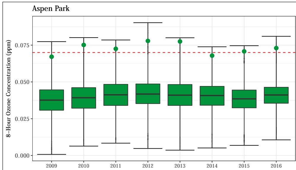
Figure 4.40: 8-hour average O 3 concentrations at the Aspen Park station. The 8-hour standard (0.070 ppm) is shown as a dashed red line. The annual design value (4 th highest daily maximum 8-hour average value) is shown for each year as a green point.
