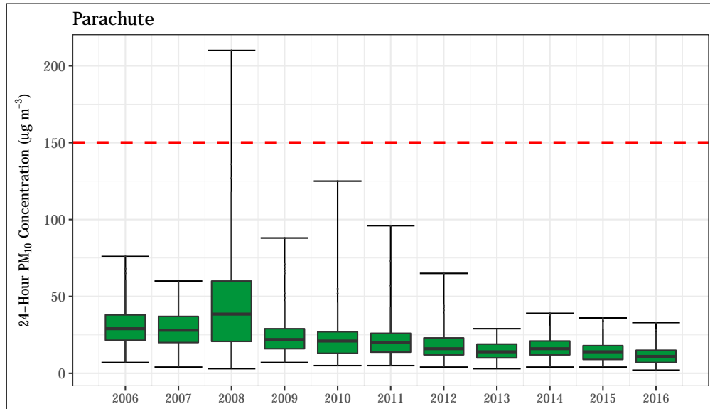
Figure 4.71: 24-hour average PM 10 concentrations at the Parachute station. The 24-hour standard (150 µg m -3 ) is shown as a dashed red line.
