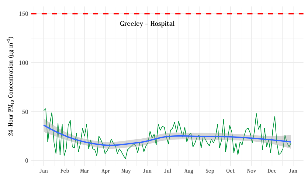
Figure 5.58: 24-hour average PM_{10} concentrations at the Greeley - Hospital station. The mean trend obtained using a generalized additive model is shown as a blue line. The 24-hour standard ( 150 \mu\text{g m}^{-3} ) is shown as a dashed red line.
