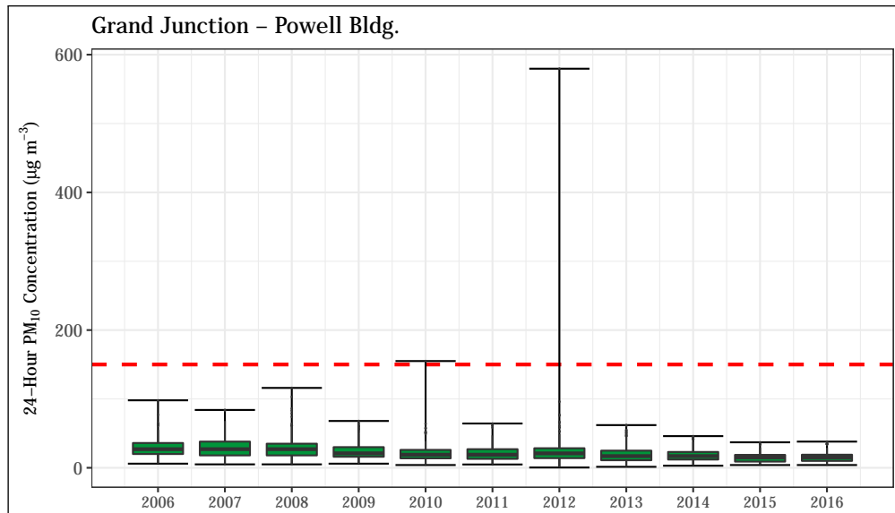
Figure 4.74: 24-hour average PM 10 concentrations at the Grand Junction - Powell Bldg. station. The 24-hour standard (150 µg m -3 ) is shown as a dashed red line.
