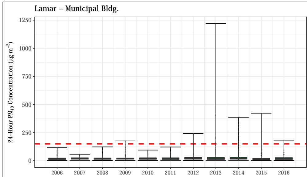
Figure 4.55: 24-hour average PM 10 concentrations at the Lamar - Municipal Bldg. station. The 24-hour standard (150 µg m -3 ) is shown as a dashed red line.
