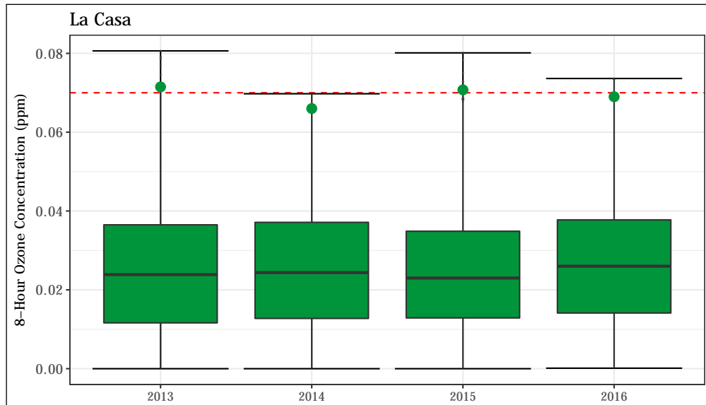
Figure 4.35: 8-hour average O 3 concentrations at the La Casa station. The 8-hour standard (0.070 ppm) is shown as a dashed red line. The annual design value (4 th highest daily maximum 8-hour average value) is shown for each year as a green point.
