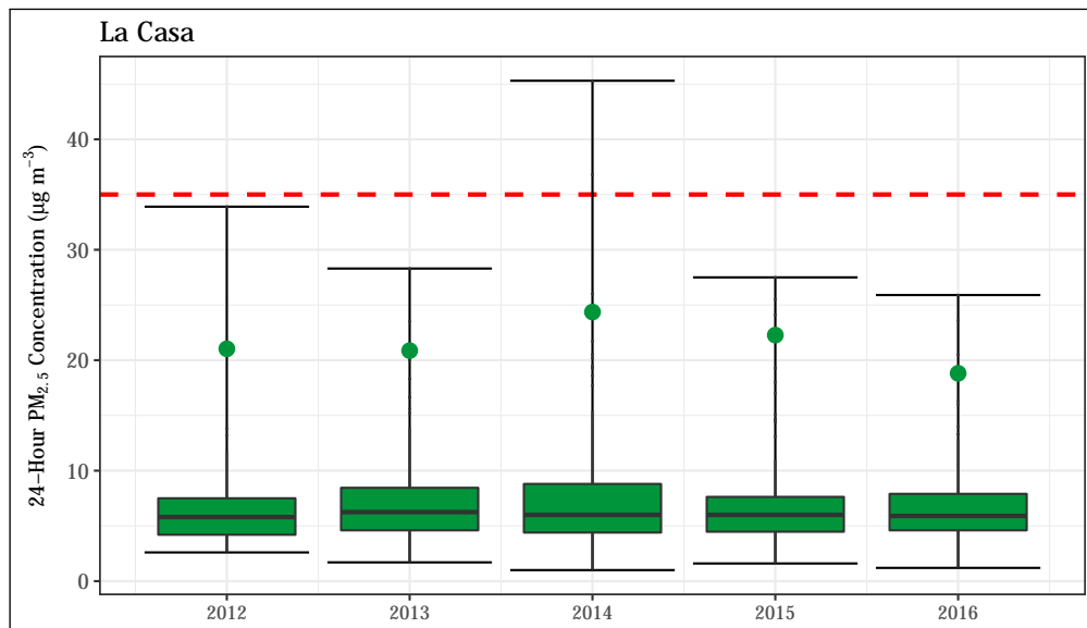
Figure 4.15: 24-hr PM 2.5 concentrations at the La Casa station. The 24-hour standard (35 µg m -3 ) is shown as a dashed red line. The annual design value (98 th percentile of values measured throughout the year) is shown for each year as a green point.
