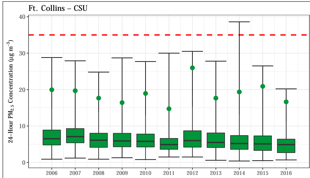
Figure 4.20: 24-hr PM 2.5 concentrations at the Ft. Collins - CSU station. The 24-hour standard (35 µg m -3 ) is shown as a dashed red line. The annual design value (98 th percentile of values measured throughout the year) is shown for each year as a green point.
