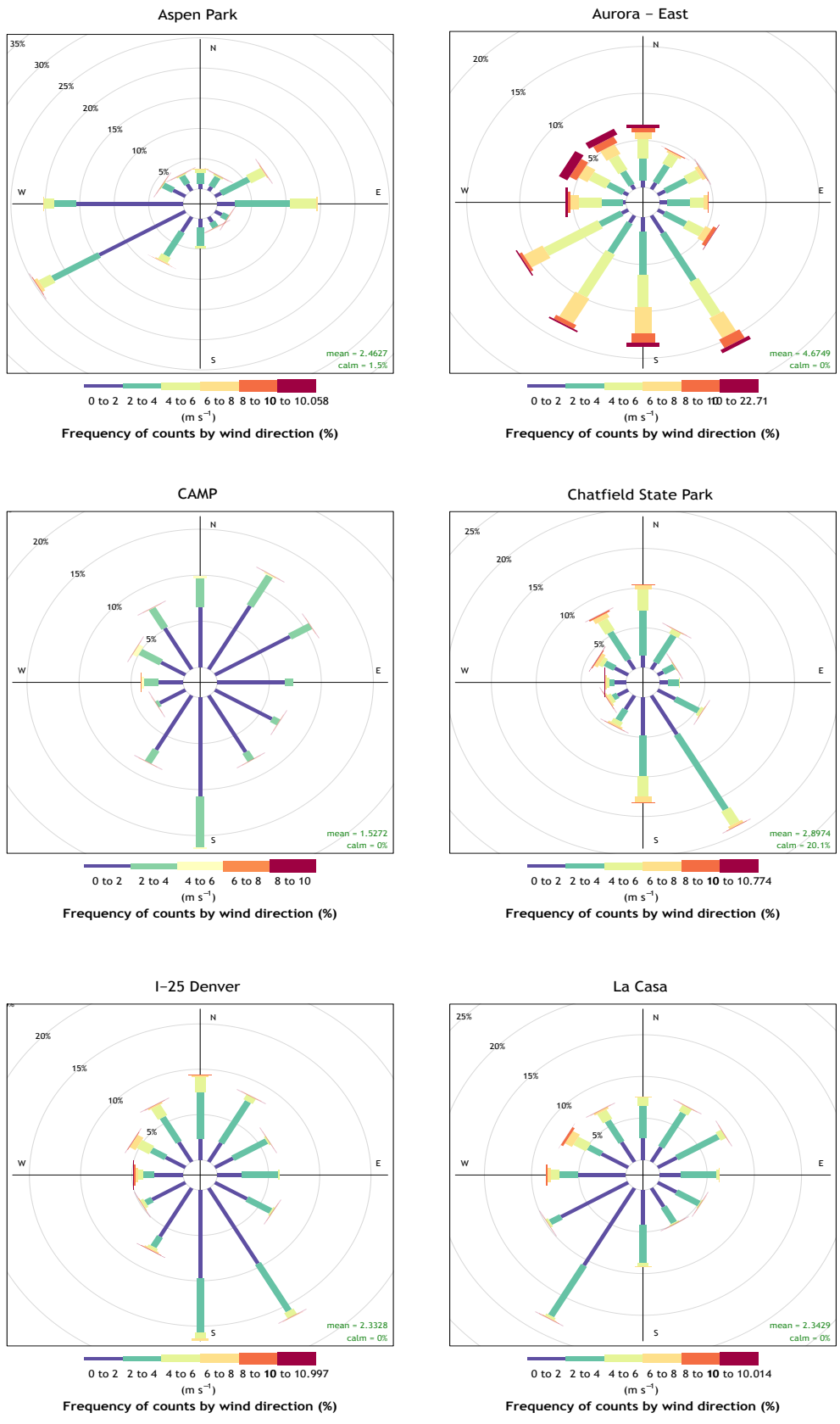
Figure 4.52: Wind roses for sites in the Denver Metro/North Front Range Region during 2016.
