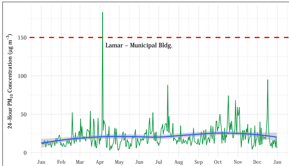
Figure 5.54: 24-hour average PM_{10} concentrations at the Lamar - Municipal Bldg. station. The mean trend obtained using a generalized additive model is shown as a blue line. The 24-hour standard ( 150 \mu\text{g m}^{-3} ) is shown as a dashed red line. The one exceedance which took place on April 5 th has been flagged by the division as an exceptional high wind event.
