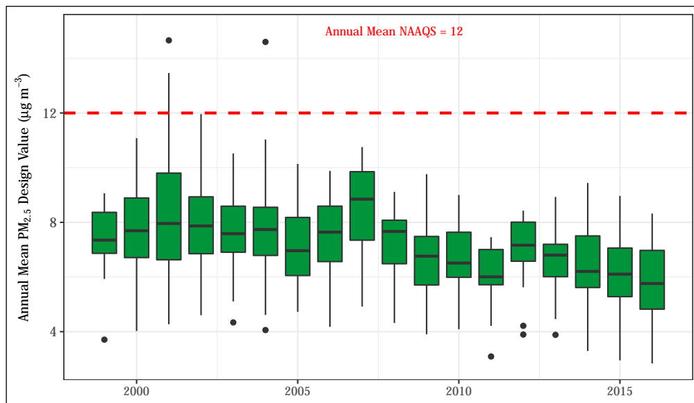
Figure 2.18: Statewide historical record of annual mean PM 2.5 design values. The box plot shows the mean design value statewide for each year, as well as the interquartile range (box) of values observed at monitoring sites throughout the state and the minimum and maximum values. Outliers are indicated by black points.
