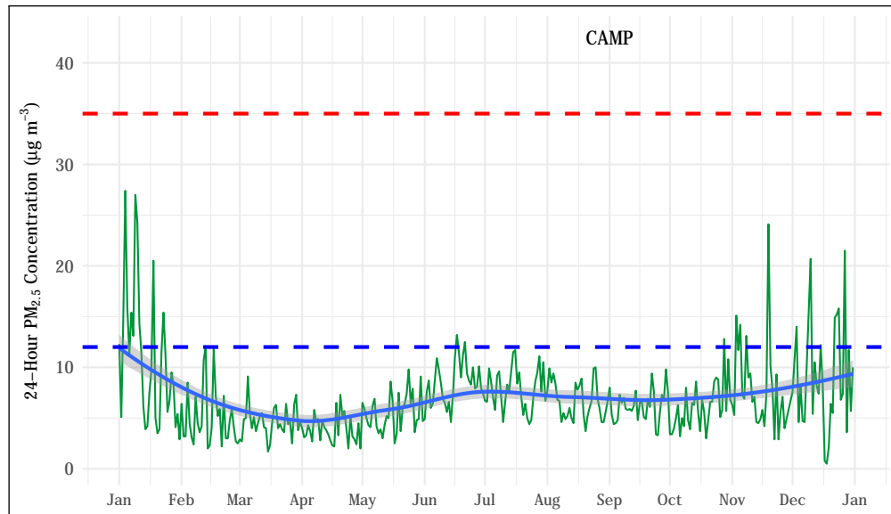
Figure 5.62: 24-hour average PM_{2.5} concentrations at the CAMP station. The mean trend obtained using a generalized additive model is shown as a blue line. The 24-hour standard ( 35 \mu\text{g m}^{-3} ) is shown as a dashed red line. The annual mean standard ( 12 \mu\text{g m}^{-3} ) is shown as a dashed blue line.
