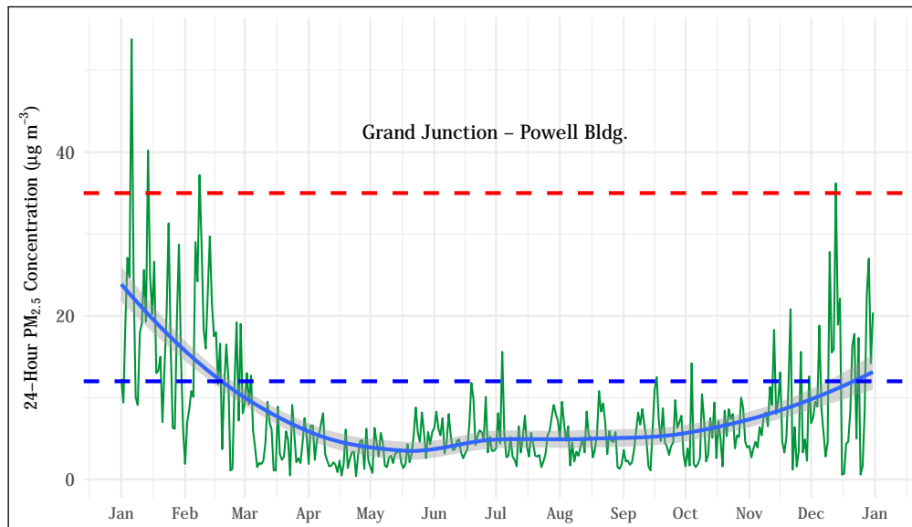
Figure 5.71: 24-hour average PM_{2.5} concentrations at the Grand Junction - Powell Bldg. GRIMM station. The mean trend obtained using a generalized additive model is shown as a blue line. The 24-hour standard ( 35 \mu\text{g m}^{-3} ) is shown as a dashed red line. The annual mean standard ( 12 \mu\text{g m}^{-3} ) is shown as a dashed blue line. The low volume particulate sampler was removed as of May, 2016, so PM_{2.5} is now recorded by use of a GRIMM continuous particulate monitor which has been in operation since January 2014. The spikes in January and December have been flagged by the division as exceptional prolonged inversion events.
