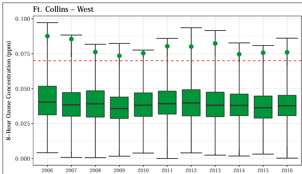
Figure 4.41: 8-hour average O 3 concentrations at the Ft. Collins - West station. The 8-hour standard (0.070 ppm) is shown as a dashed red line. The annual design value (4 th highest daily maximum 8-hour average value) is shown for each year as a green point.
