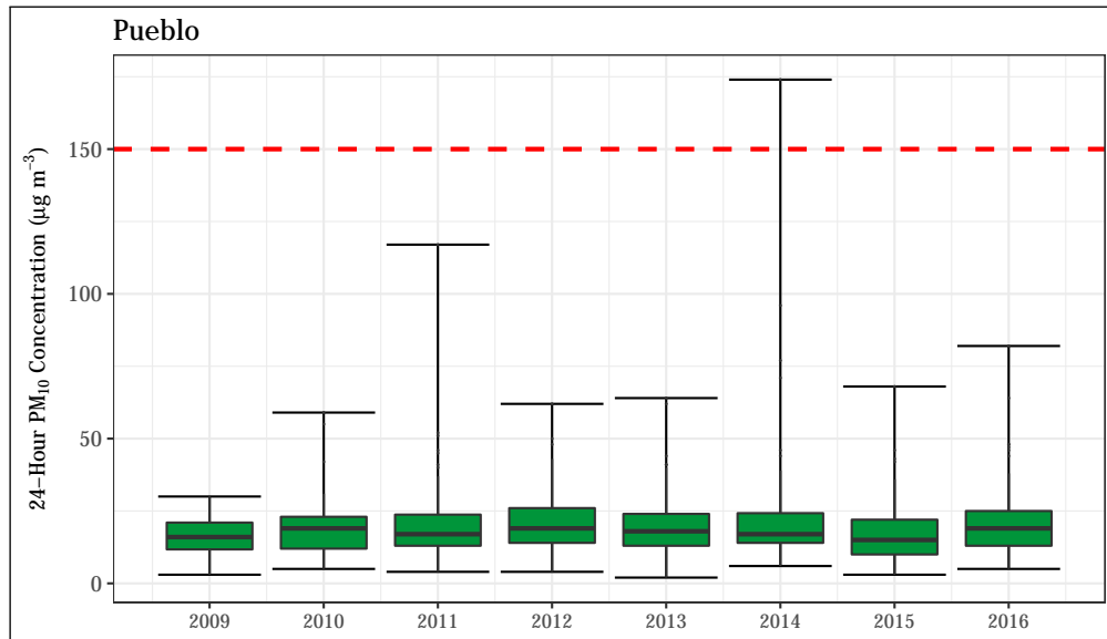
Figure 4.65: 24-hour average PM 10 concentrations at the Pueblo station. The 24-hour standard (150 µg m -3 ) is shown as a dashed red line.
