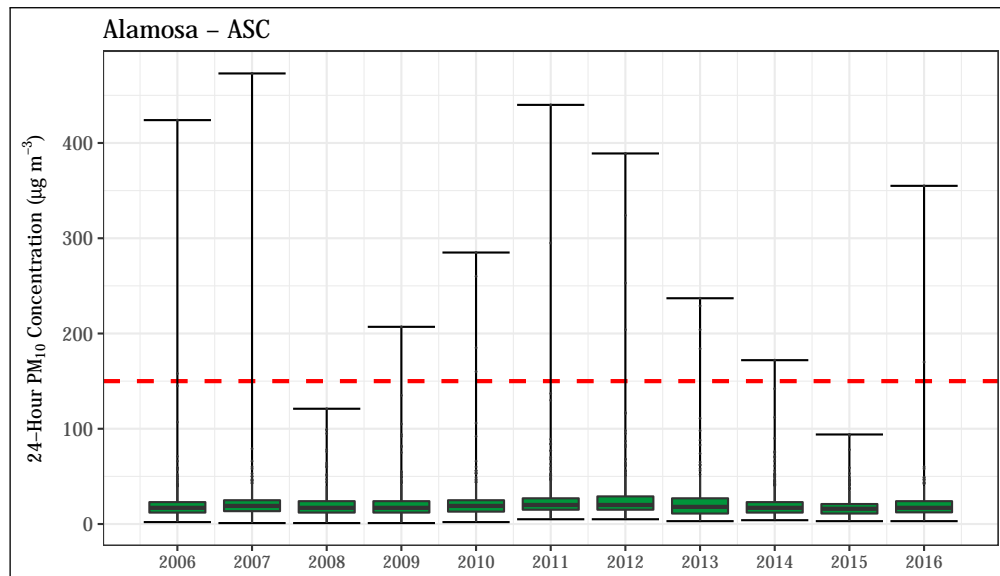
Figure 4.63: 24-hour average PM 10 concentrations at the Alamosa - ASC station. The 24-hour standard (150 µg m -3 ) is shown as a dashed red line.
