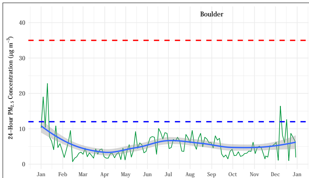
Figure 5.61: 24-hour average PM_{2.5} concentrations at the Boulder Chamber of Commerce station. The mean trend obtained using a generalized additive model is shown as a blue line. The 24-hour standard ( 35 \mu\text{g m}^{-3} ) is shown as a dashed red line. The annual mean standard ( 12 \mu\text{g m}^{-3} ) is shown as a dashed blue line.
