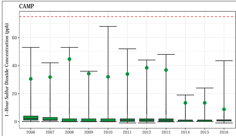
Figure 4.50: 1-hour average SO 2 concentrations at the CAMP station. The annual design value (99 th percentile of daily maximum 1-hour values) is shown for each year as a green point.
