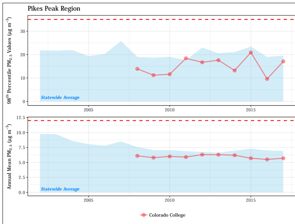
Figure 4.31: Fifteen-year trend in 24-hour PM 2.5 annual 98 th percentile values (top) and annual mean concentrations (bottom) for monitoring sites in the Pikes Peak region. The 24-hour and annual mean NAAQS (35 µg m -3 and 12 µg m -3 , respectively) are shown as dashed red lines.
