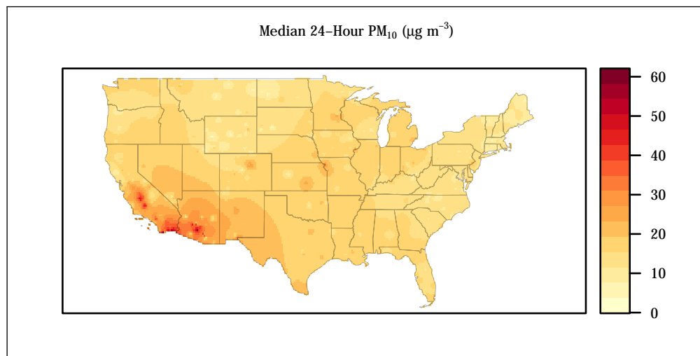
Figure 2.21: Interpolation map of median 24-hour PM_{10} values for air quality monitoring stations in the continental U.S. during 2017
