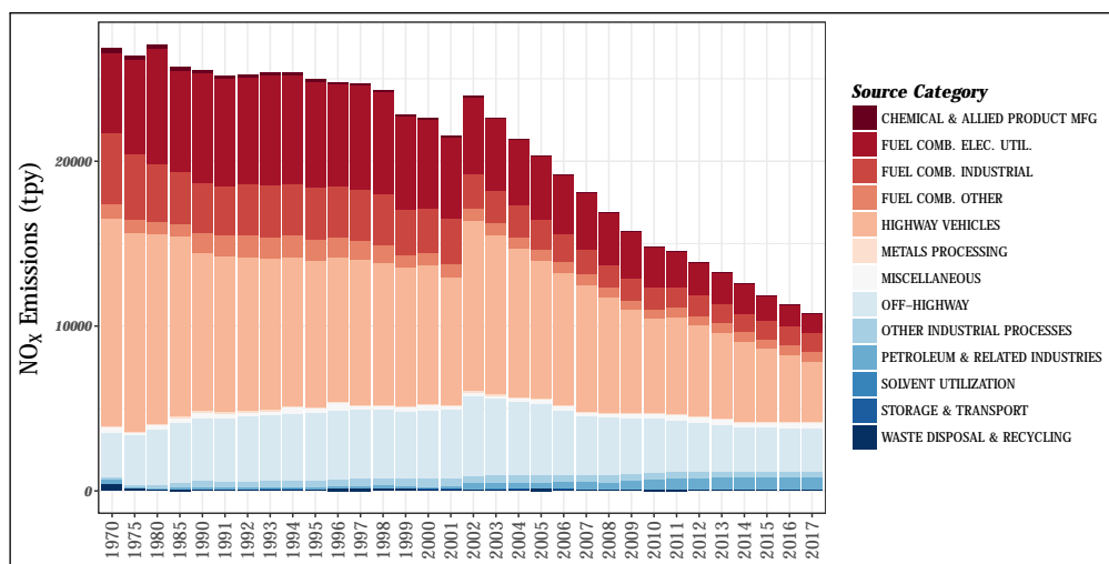
Figure 2.13: Trends in national NO x emissions from 1970 to 2017.
