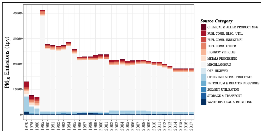
Figure 2.18: Trends in national PM 10 emissions from 1970 to 2017.
