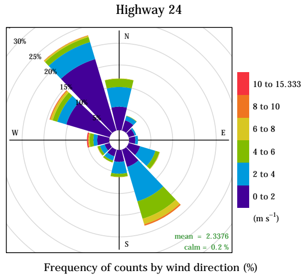
Figure 4.35: Wind rose from the Highway 24 meteorological station.
