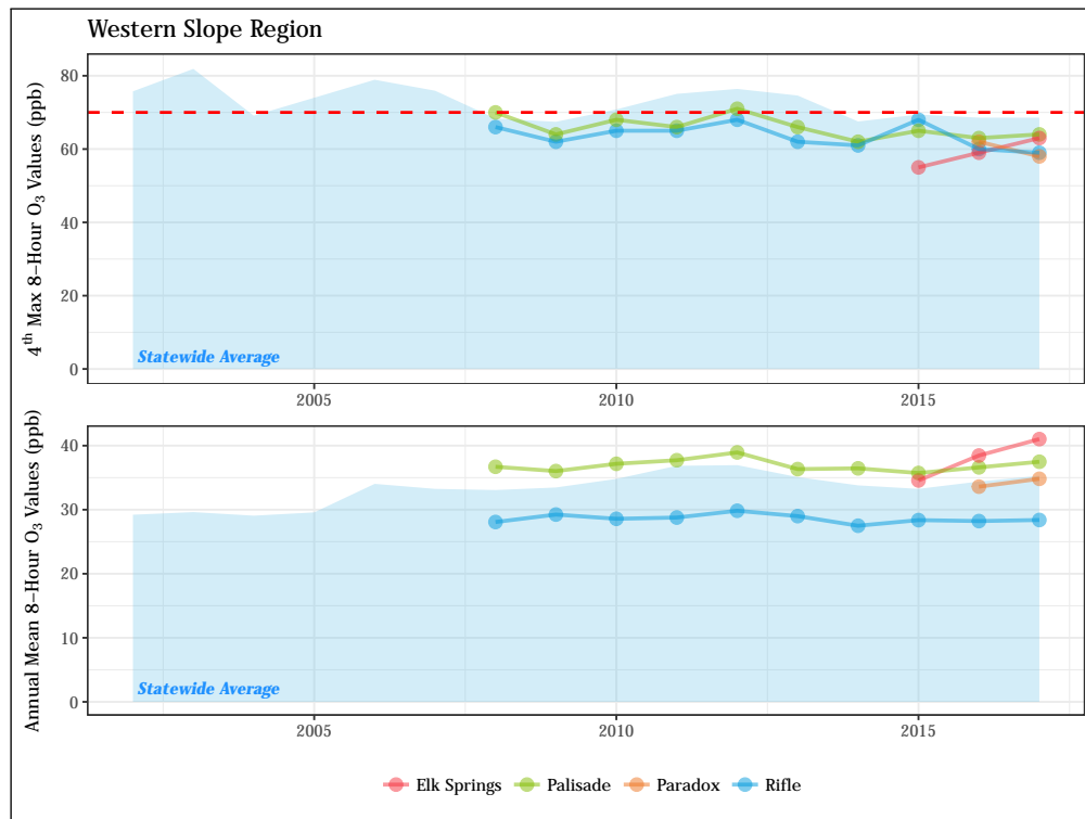
Figure 4.44: Fifteen-year trend in ozone eight-hour NAAQS values (top) and annual mean eight-hour concentrations (bottom) for monitoring sites in the Western Slope region. The eight-hour NAAQS (70 ppb) is shown as a dashed red line.
