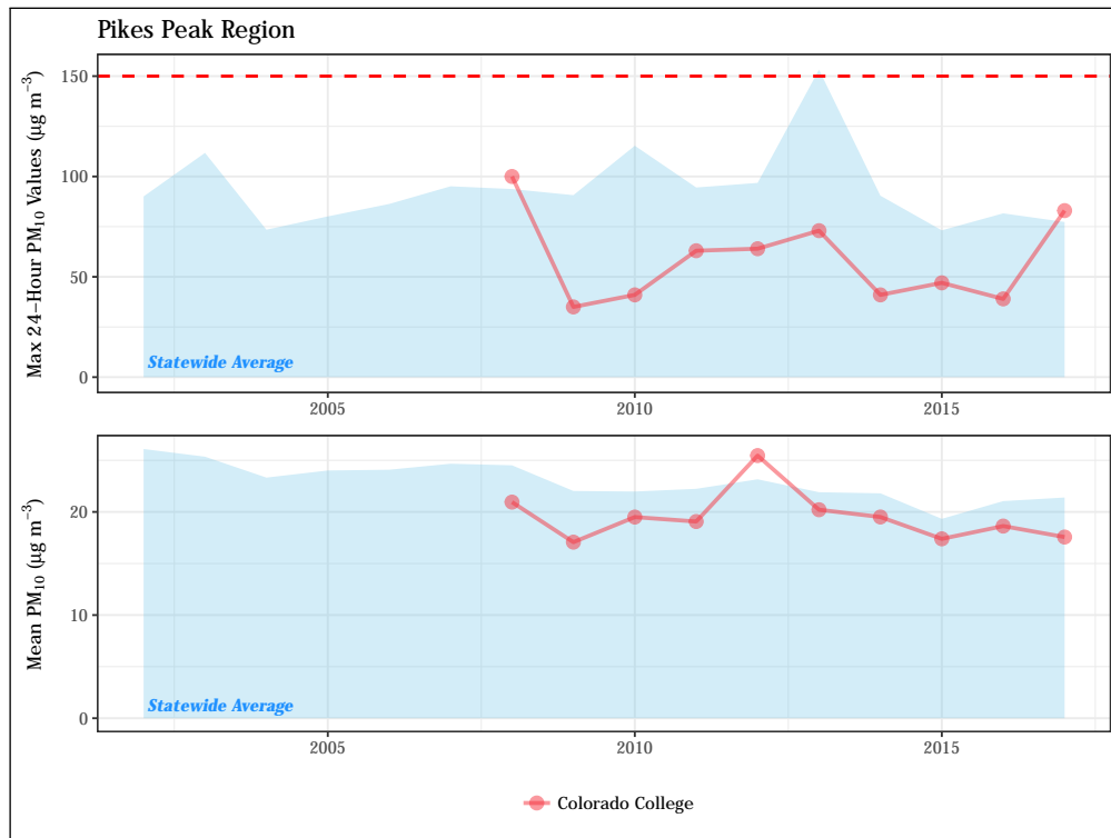
Figure 4.30: Fifteen-year trend in maximum 24-hour PM 10 values (top) and annual mean concentrations (bottom) for monitoring sites in the Pikes Peak region. The 24-hour NAAQS (150 µg m -3 ) is shown as a dashed red line.
