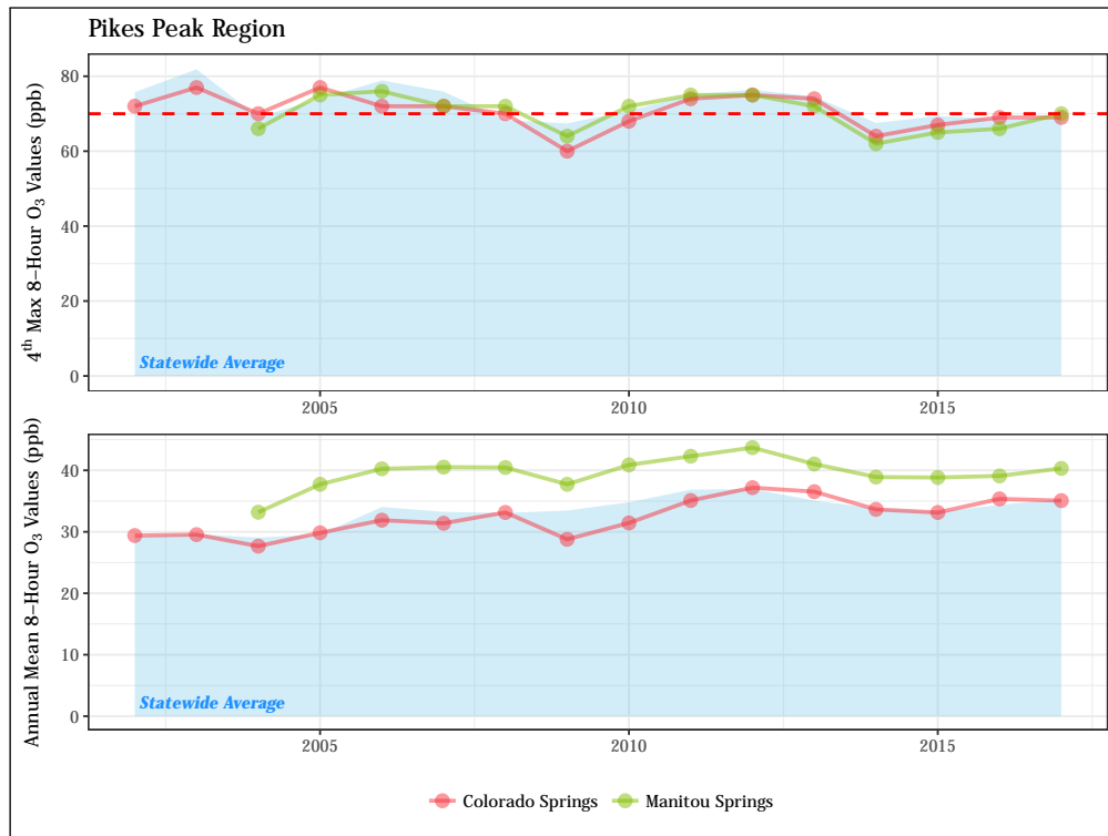
Figure 4.33: Fifteen-year trend in ozone eight-hour NAAQS values (top) and annual mean eight-hour concentrations (bottom) for monitoring sites in the Pikes Peak region. The eight-hour NAAQS (70 ppb) is shown as a dashed red line.
