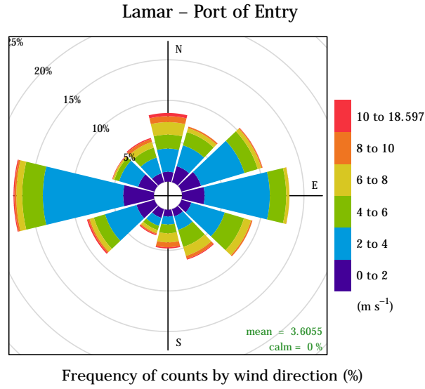
Figure 4.29: Wind rose from the Lamar - Port of Entry meteorological station.
