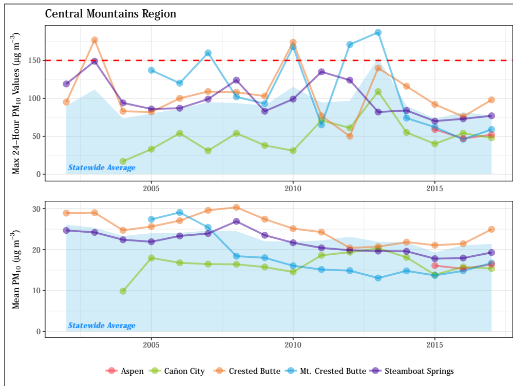
Figure 4.1: Fifteen-year trend in maximum 24-hour PM 10 values (top) and annual mean concentrations (bottom) for monitoring sites in the Central Mountains region. The 24-hour NAAQS ( 150 \mu\text{g m}^{-3} ) is shown as a dashed red line.
