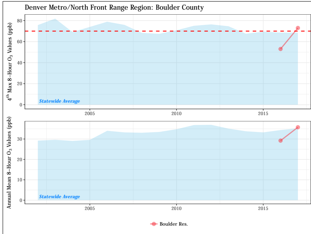
Figure 4.17: Fifteen-year trend in ozone eight-hour NAAQS values (top) and annual mean eight-hour concentrations (bottom) for monitoring sites in Denver Boulder. The eight-hour NAAQS (70 ppb) is shown as a dashed red line.
