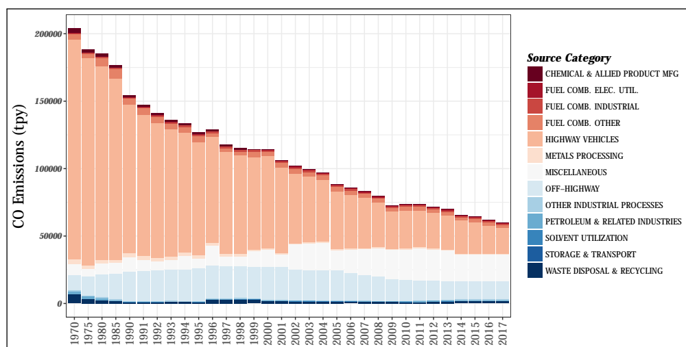
Figure 2.1: Trends in national carbon monoxide emissions from 1970 to 2017.
