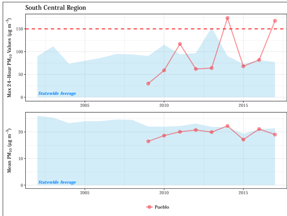
Figure 4.37: Fifteen-year trend in maximum 24-hour PM 10 values (top) and annual mean concentrations (bottom) for monitoring sites in the South Central region. The 24-hour NAAQS (150 µg m -3 ) is shown as a dashed red line.
