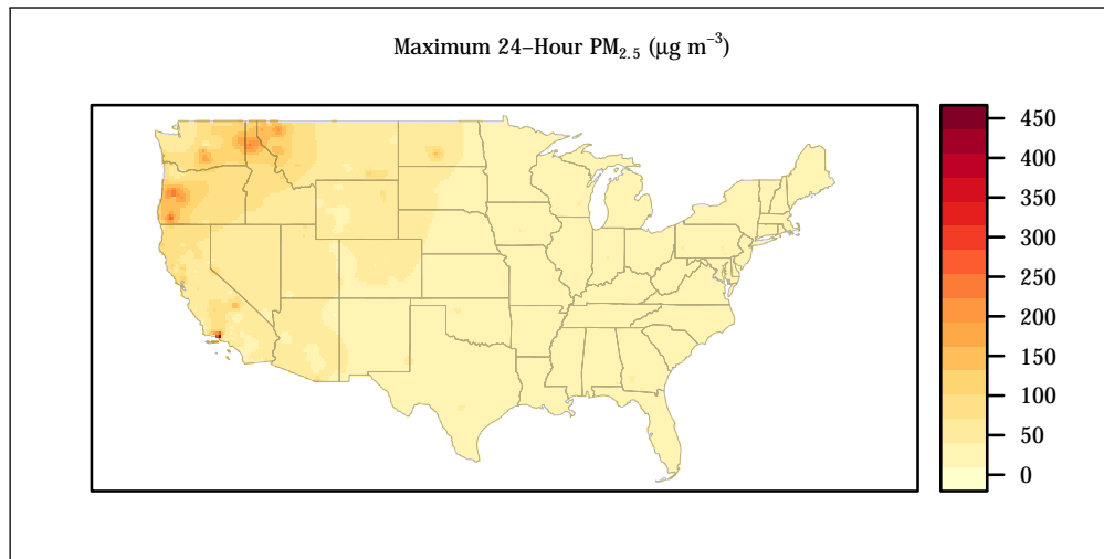
Figure 2.24: Interpolation map of maximum 24-hour PM 2.5 values for air quality monitoring stations in the continental U.S. during 2017
