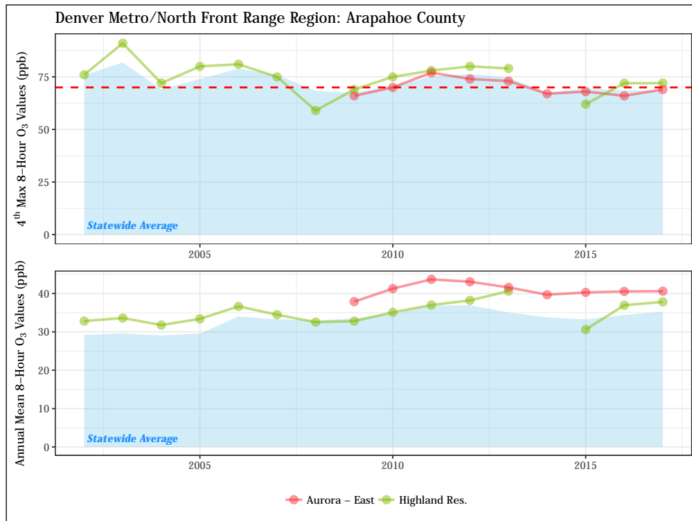
Figure 4.16: Fifteen-year trend in ozone eight-hour NAAQS values (top) and annual mean eight-hour concentrations (bottom) for monitoring sites in Denver Arapahoe. The 8-hour NAAQS (70 ppb) is shown as a dashed red line.
