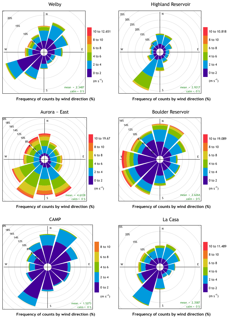
Figure 4.25: Wind roses for sites in the Denver Metro/North Front Range Region during 2017.
