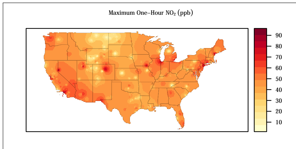
Figure 2.17: Interpolation map of maximum one-hour NO 2 values for air quality monitoring stations in the continental U.S. during 2017
