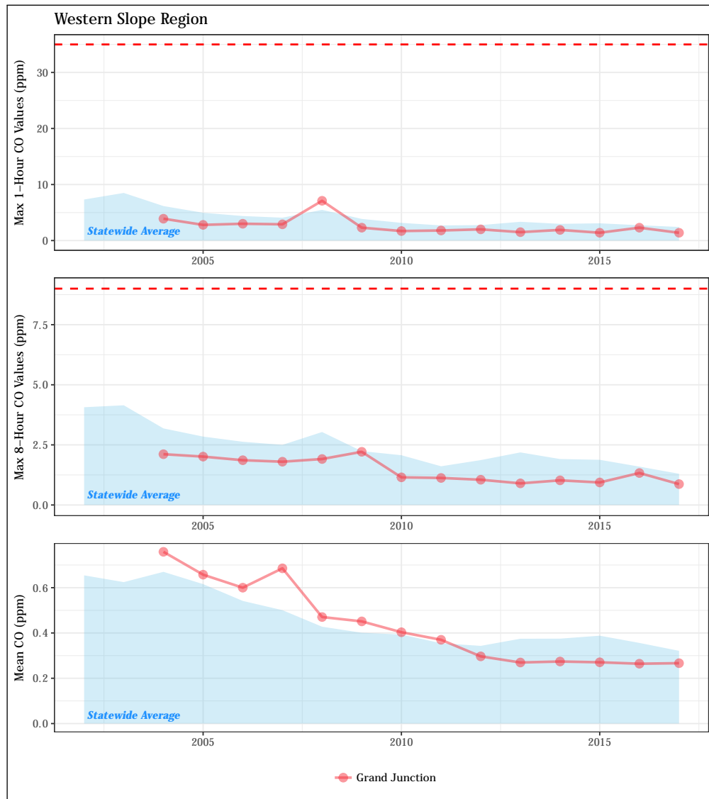
Figure 4.43: Fifteen-year trend in annual maximum one-hour (top) and eight-hour (center) CO values and annual mean eight-hour CO concentrations (bottom) for monitoring sites in the Western Slope region. The one-hour and eight-hour NAAQS (35 ppm and 9 ppm, respectively) are shown as dashed red lines.
