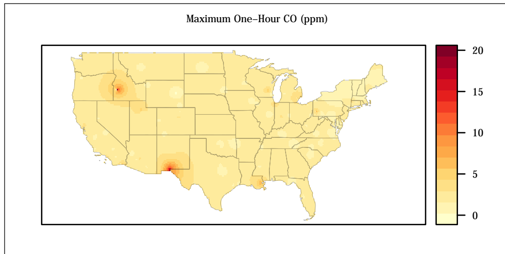
Figure 2.5: Interpolation map of maximum one-hour CO values for air quality monitoring stations in the continental U.S. during 2017
