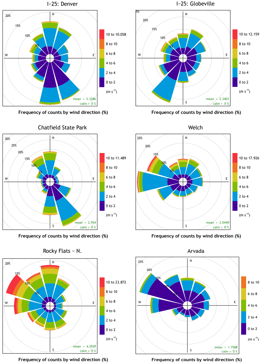
Figure 4.26: Wind roses for sites in the Denver Metro/North Front Range Region during 2017 (continued).
