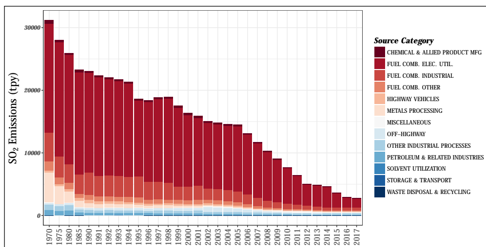
Figure 2.6: Trends in national sulfur dioxide emissions from 1970 to 2017.
