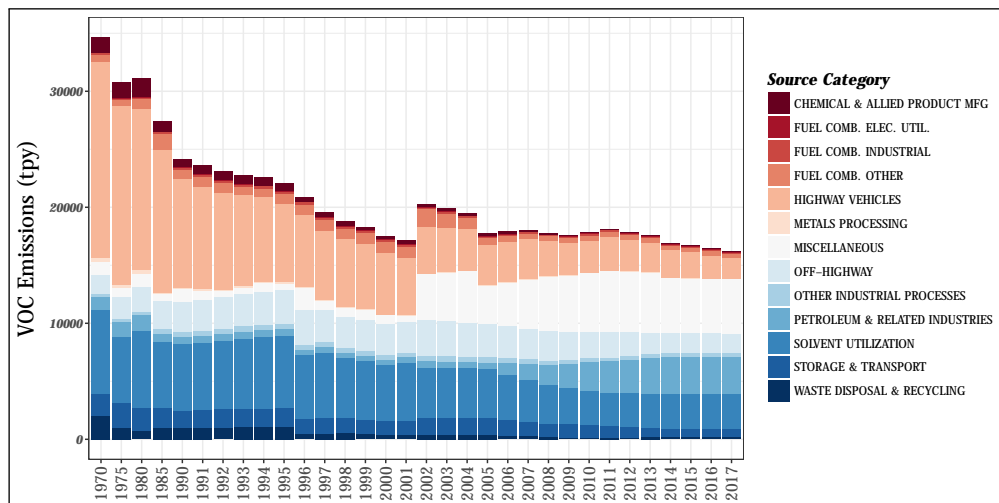
Figure 2.10: Trends in national VOC emissions from 1970 to 2017.
