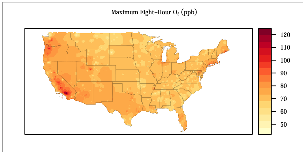
Figure 2.12: Interpolation map of maximum eight-hour O 3 values for air quality monitoring stations in the continental U.S. during 2017
