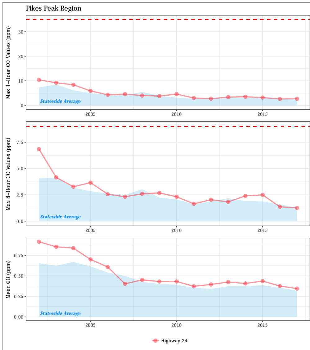
Figure 4.32: Fifteen-year trend in annual maximum one-hour (top) and eight-hour (center) CO values and annual mean eight-hour CO concentrations (bottom) for monitoring sites in the Pikes Peak region. The one-hour and eight-hour NAAQS (35 ppm and 9 ppm, respectively) are shown as dashed red lines.
