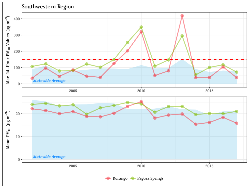
Figure 4.39: Fifteen-year trend in maximum 24-hour PM 10 values (top) and annual mean concentrations (bottom) for monitoring sites in the Southwest region. The 24-hour NAAQS (150 µg m -3 ) is shown as a dashed red line.
