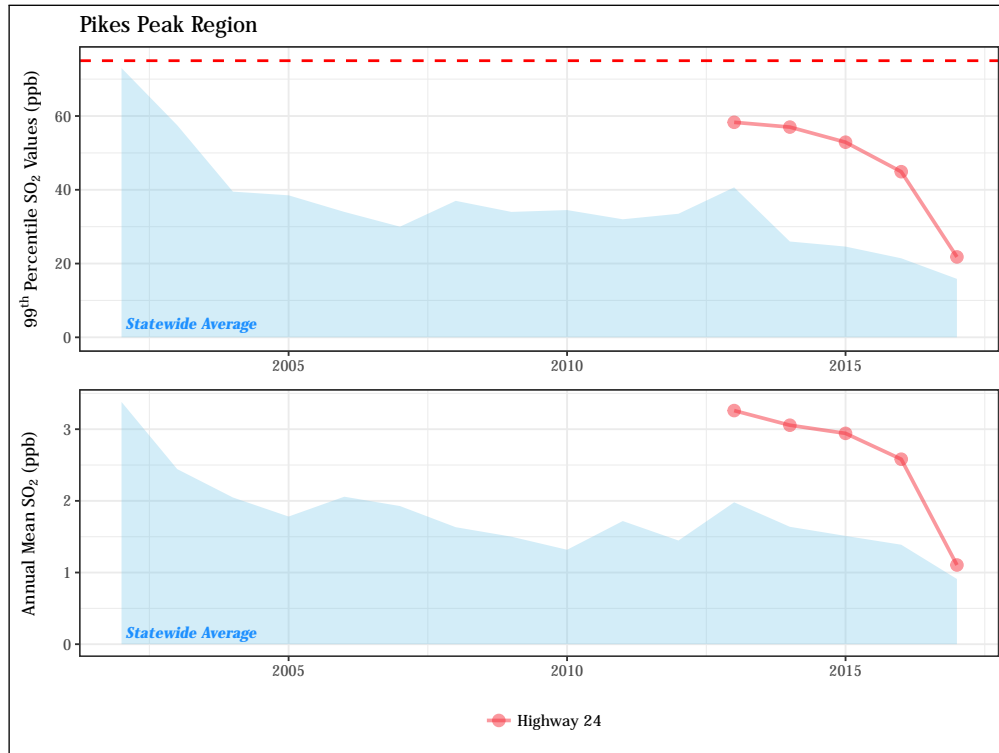
Figure 4.34: Fifteen-year trend in sulfur dioxide one-hour NAAQS values (top) and annual mean one-hour concentrations (bottom) for monitoring sites in the Pikes Peak region. The one-hour NAAQS (75 ppb) is shown as a dashed red line.
