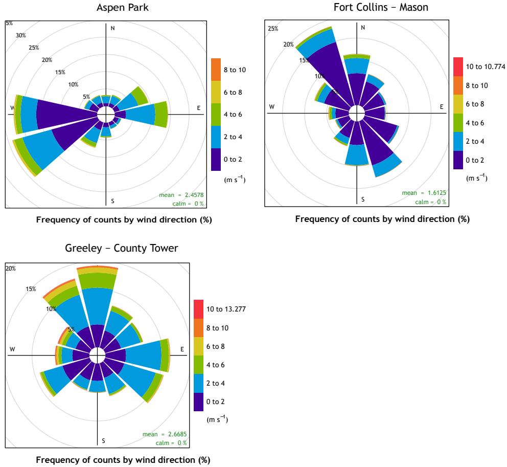
Figure 4.27: Wind roses for sites in the Denver Metro/North Front Range Region during 2017 (continued).
