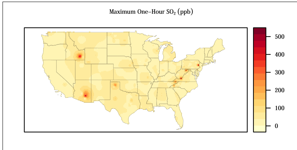
Figure 2.9: Interpolation map of maximum one-hour SO 2 values for air quality monitoring stations in the continental U.S. during 2017
