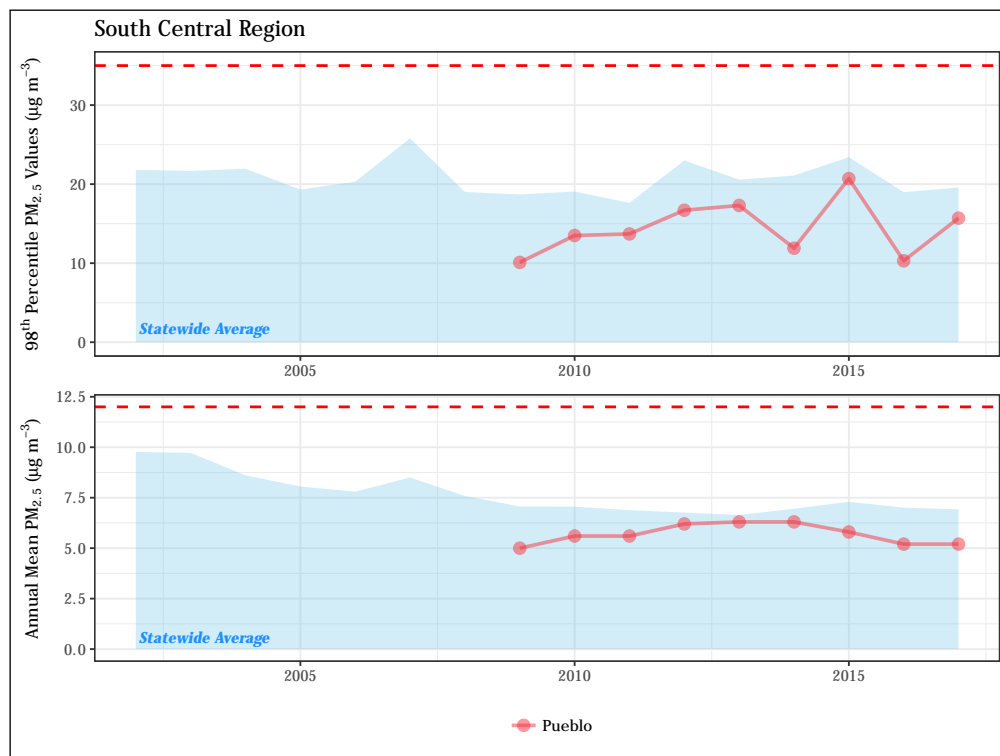
Figure 4.38: Fifteen-year trend in 24-hour PM 2.5 annual 98 th percentile values (top) and annual mean concentrations (bottom) for monitoring sites in the South Central region. The 24-hour and annual mean NAAQS (35 µg m -3 and 12 µg m -3 , respectively) are shown as dashed red lines.
