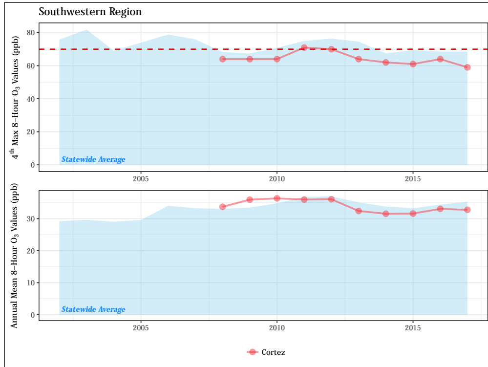
Figure 4.40: Fifteen-year trend in ozone eight-hour NAAQS values (top) and annual mean eight-hour concentrations (bottom) for monitoring sites in the Southwest region. The eight-hour NAAQS (70 ppb) is shown as a dashed red line.
