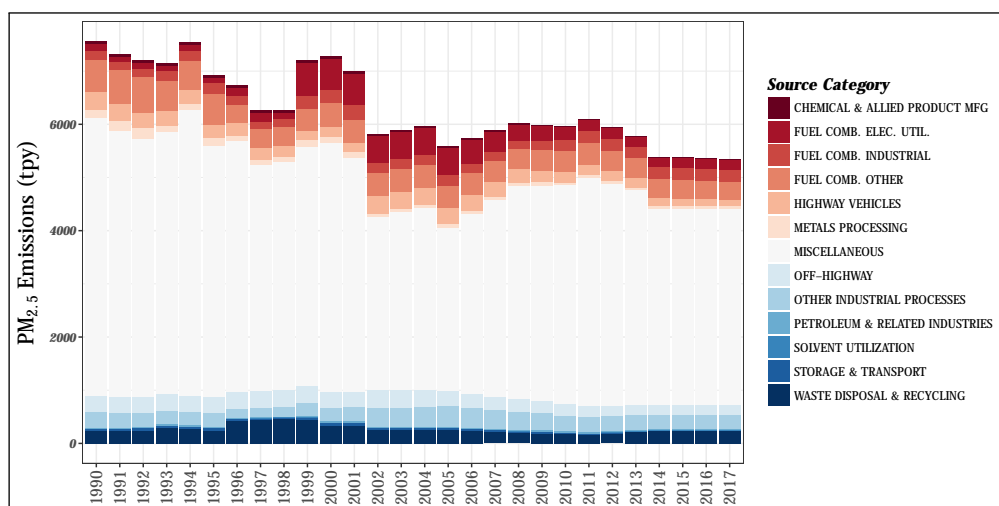
Figure 2.19: Trends in national PM 2.5 emissions from 1990 to 2017.
