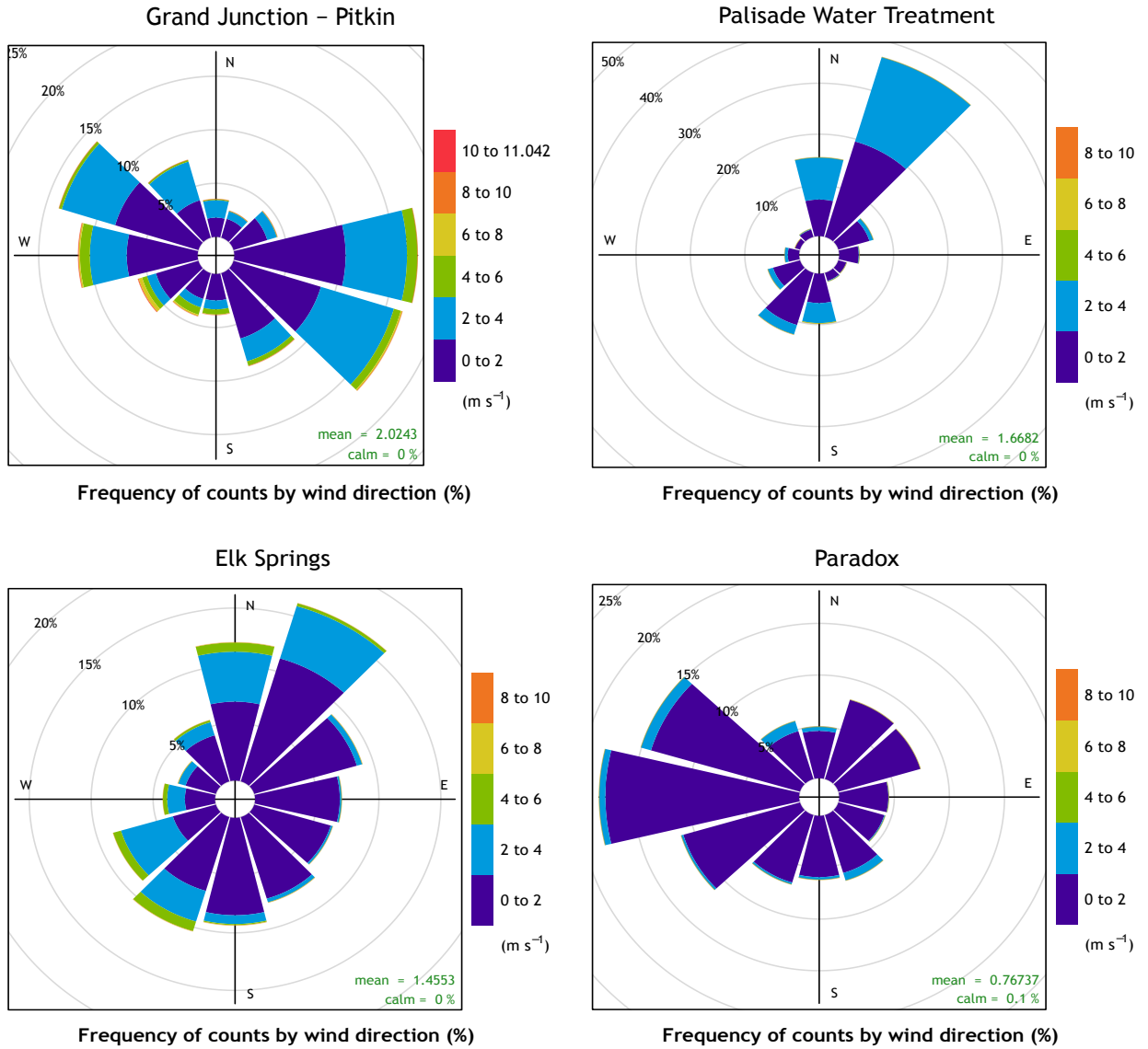
Figure 4.45: Wind roses for sites in the Western Slope Region during 2017.
