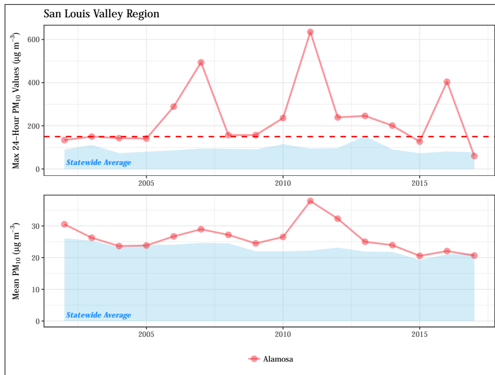
Figure 4.36: Fifteen-year trend in maximum 24-hour PM 10 values (top) and annual mean concentrations (bottom) for monitoring sites in the San Luis Valley region. The 24-hour NAAQS (150 µg m -3 ) is shown as a dashed red line.
