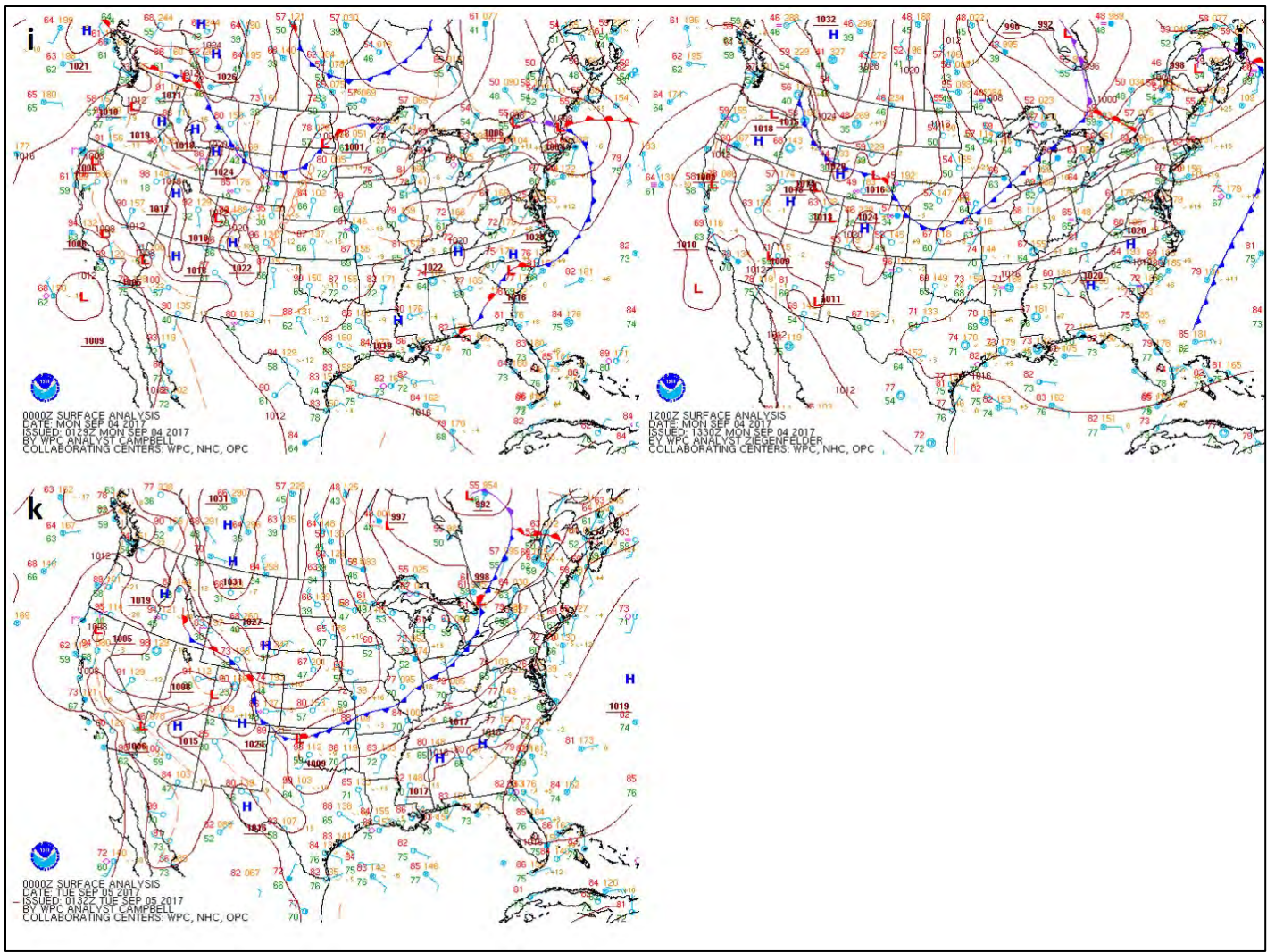
Figures 12i-k: NOAA surface analysis at (i) 5:00 PM MST (OZ September 4, 2017) September 3, 2017; (j) 5:00 AM MST (12Z) September 4, 2017; (k) 5:00 PM MST (OZ September 5, 2017) September 4, 2017. (source: http://www.wpc.ncep.noaa.gov/ )
