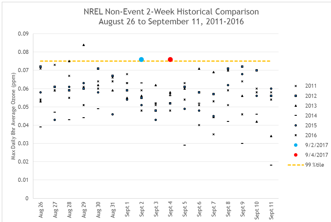
Figure 51: 2-Week Non-Event Historical Comparison Plots for Highland (AQS ID 080050002) and NREL (AQS ID 080590011)
