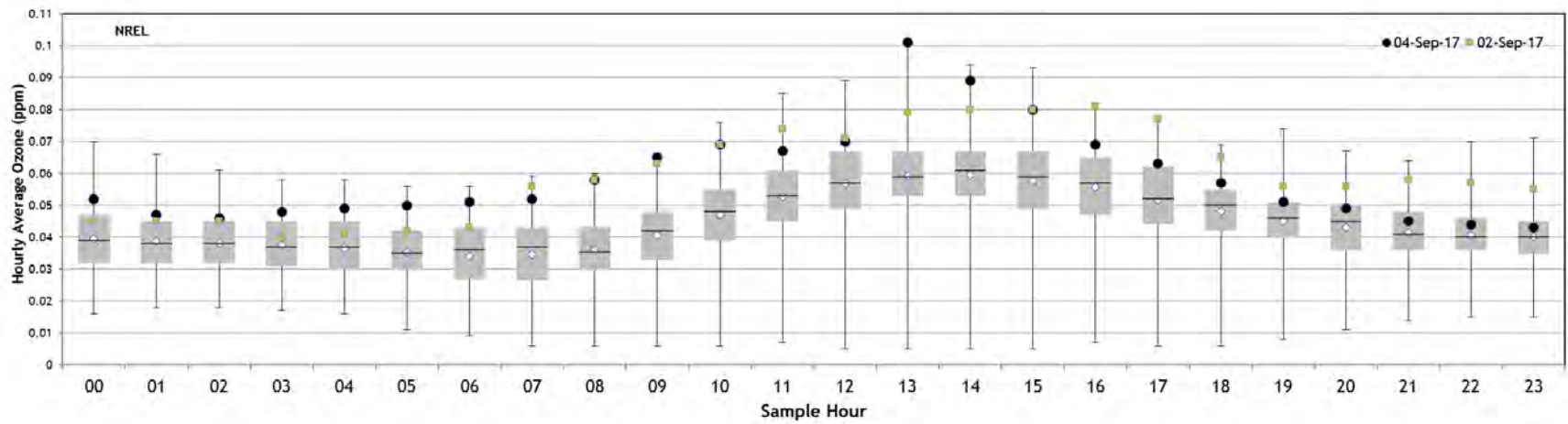
Figure 53: Diurnal Deviation from Normal Plots for hourly data at Highland (AQS ID 080050002) and NREL (AQS ID 080590011)
