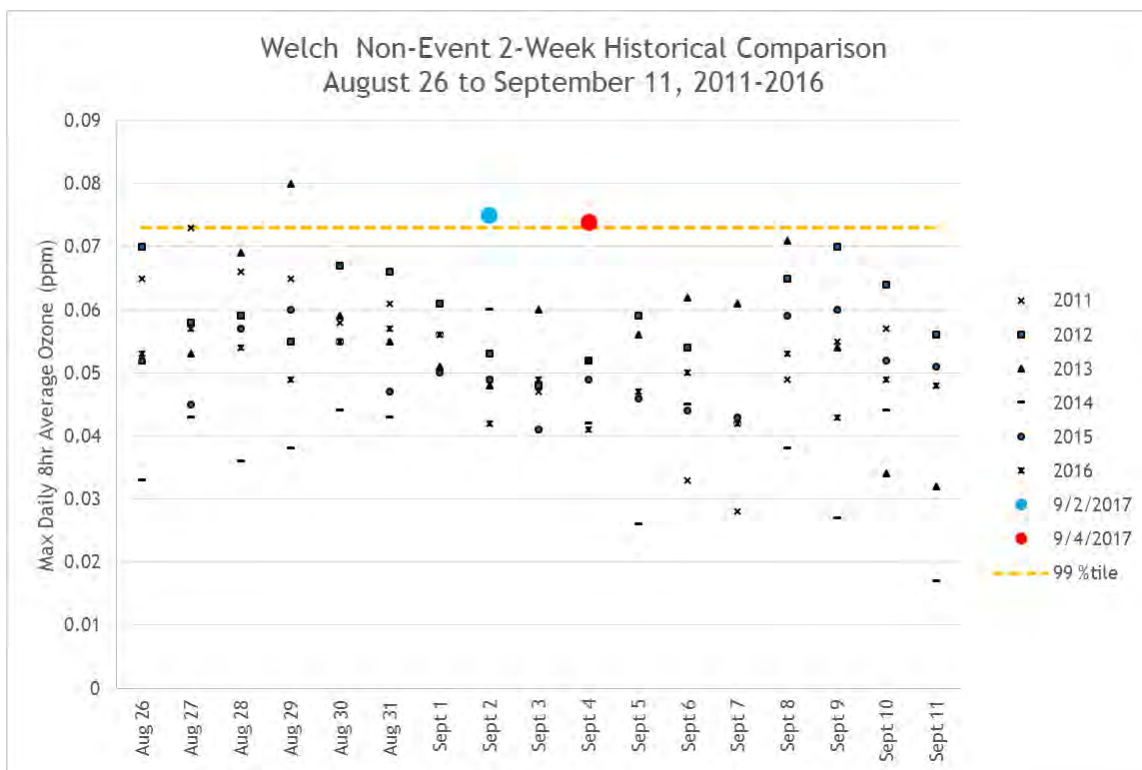
Figure 52: 2-Week Non-Event Historical Comparison Plots for RFN (AQS ID 080590006) and Welch (AQS ID 080590005)
