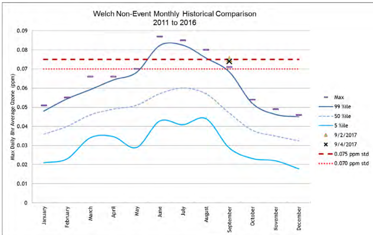
Figure 49: Monthly Non-Event Historical Comparison Plots for RFN (AQS ID 080590006) and Welch (AQS ID 080590005)
