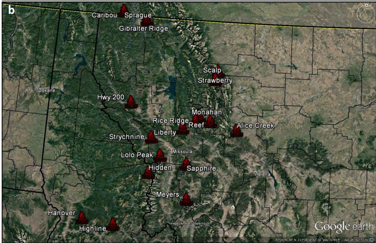
Figures 39a-b: Active wildfires on September 2, 2017 in (a) central Washington, and (b) northern Idaho and western Montana.
