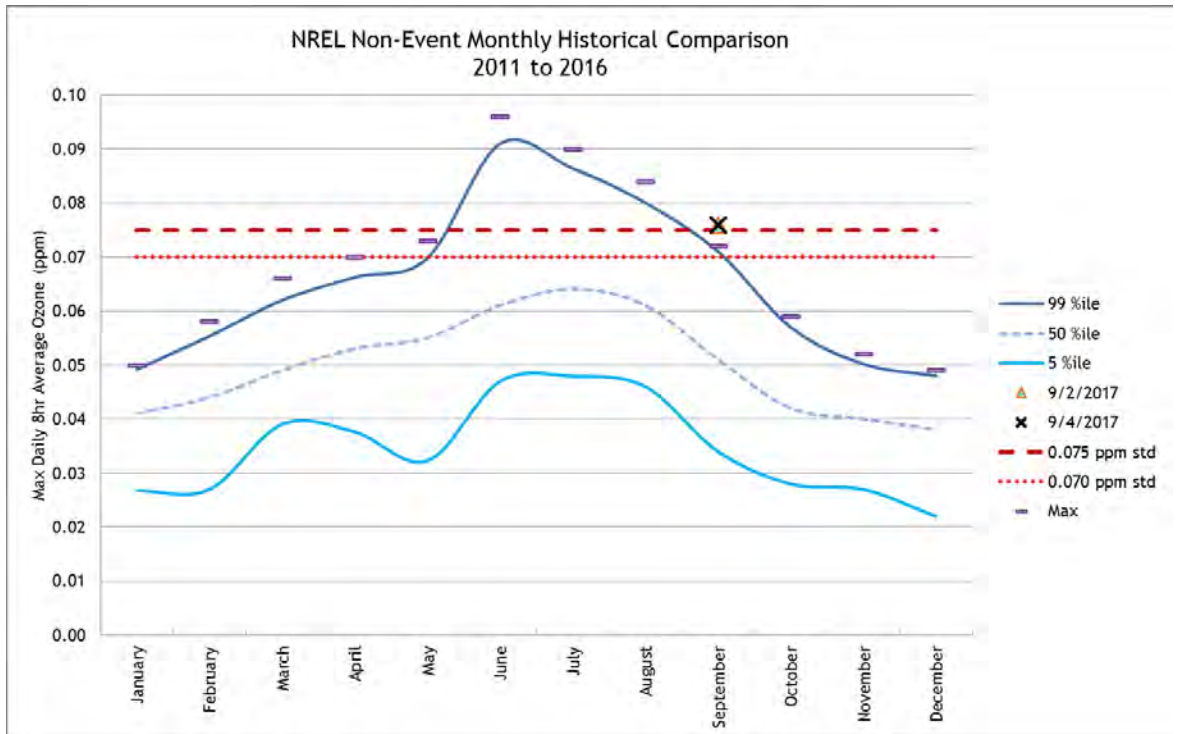
Figure 48: Monthly Non-Event Historical Comparison Plots for Highland (AQS ID 080050002) and NREL (AQS ID 080590011)
