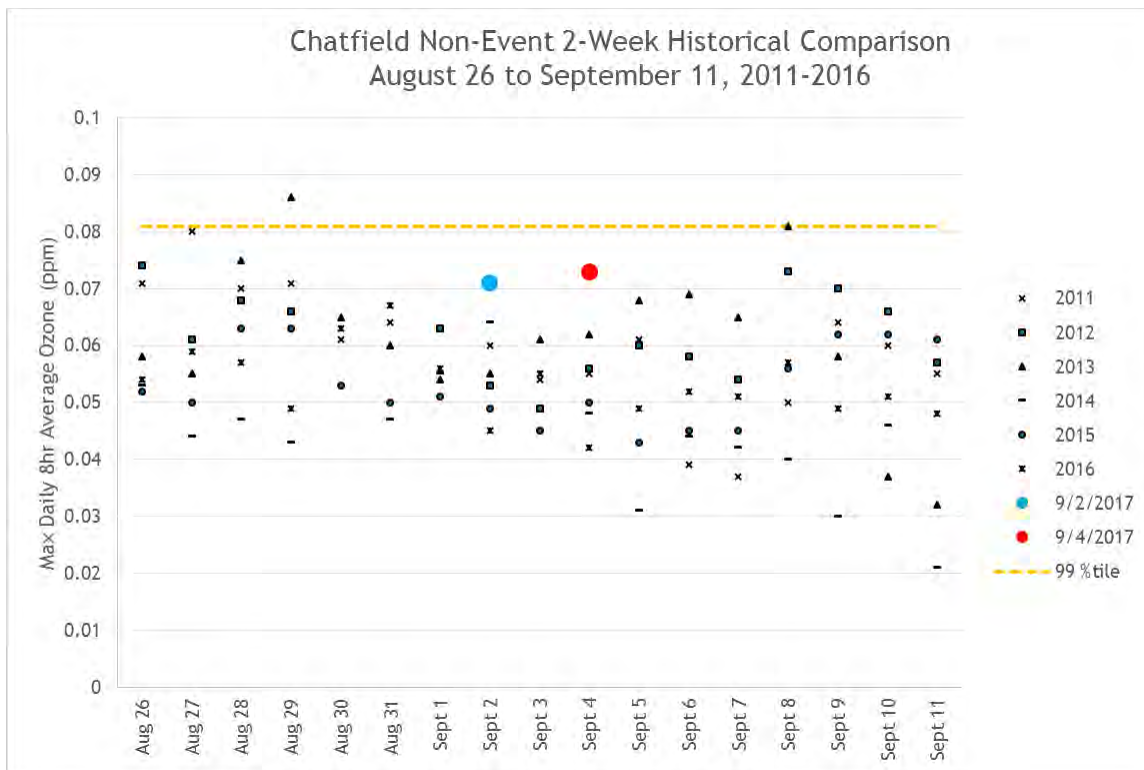
Figure 50: 2-Week Non-Event Historical Comparison Plots for Aspen Park (AQS ID 080590013) and Chatfield (AQS ID 080350004)
