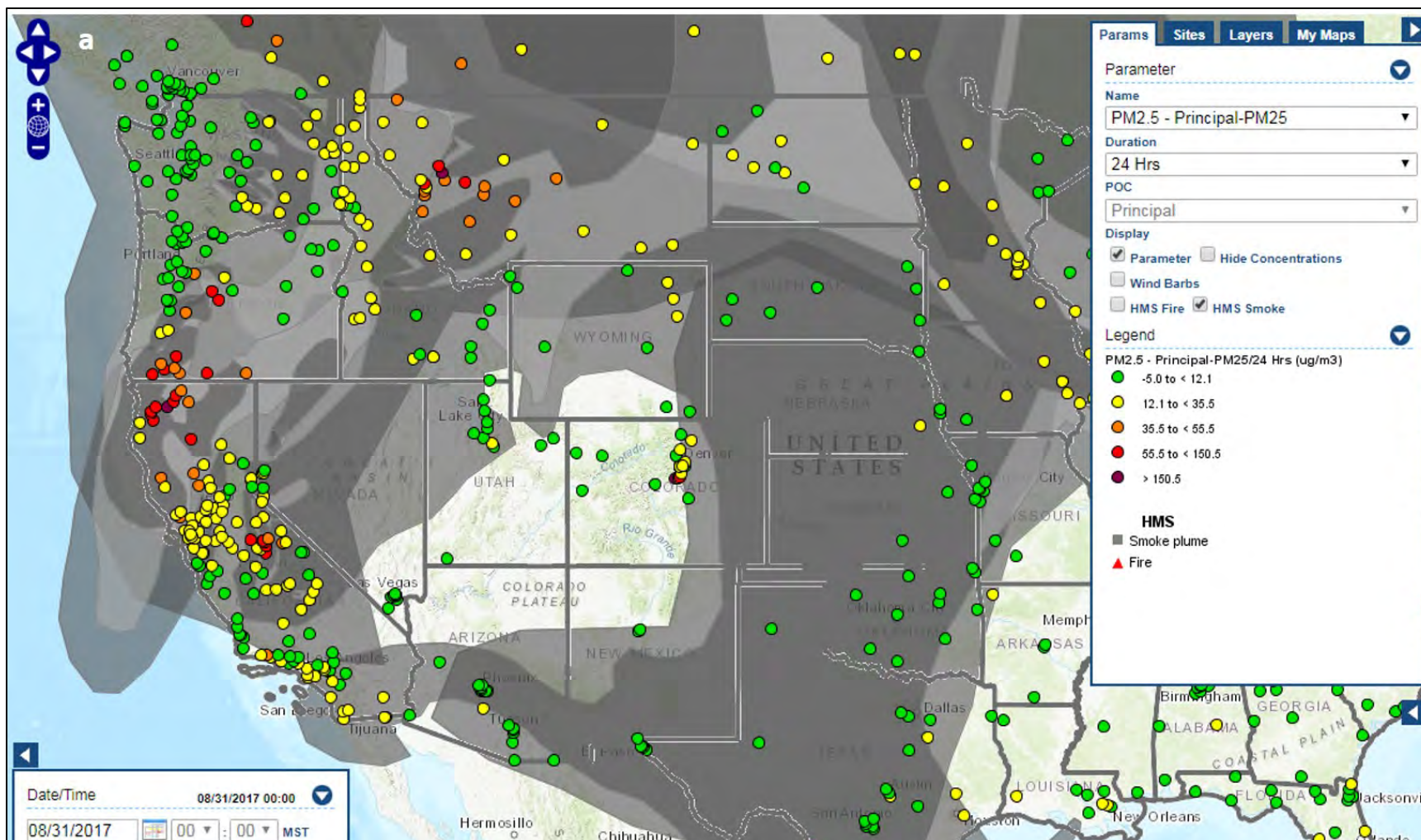
Figure 18a: HMS Smoke detection and 24-hr average PM 2.5 concentration on August 31, 2017. (source: https://airnowtech.org/navigator )
