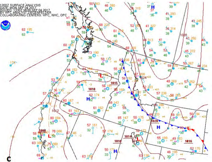
Figures 43a-d: NOAA surface analysis for northwestern US at (a) 5:00 AM MST (12z) on September 3, 2017, (b) 5:00 PM MST (OZ 9/4/2017) on September 3, 2017, (c) 5:00 AM MST (12Z) on September 4, 2017, and (d) 5:00 PM MST (OZ 9/5/2017) on September 4, 2017 (source: http://www.wpc.ncep.noaa.gov/ )
