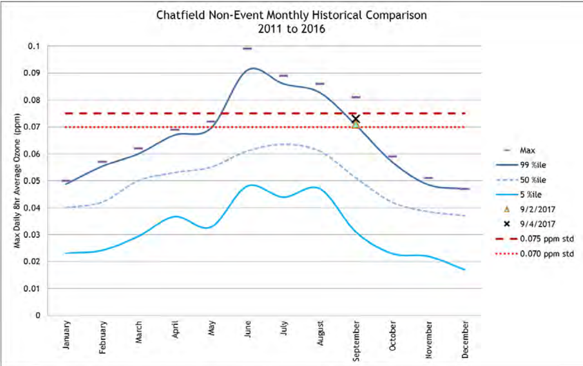
Figure 47: Monthly Non-Event Historical Comparison Plots for Aspen Park (AQS ID 080590013) and Chatfield (AQS ID 080350004)
